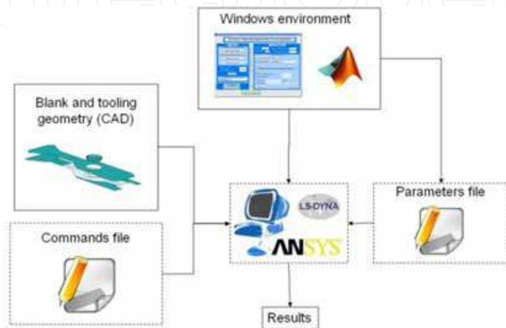
Fig. 4. Automation procedure
