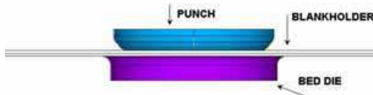
Fig. 1. Starting situation of the dies
