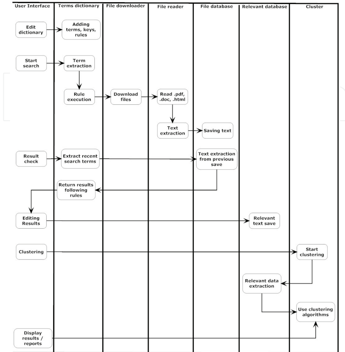
Fig. 5. IRS activities diagram
