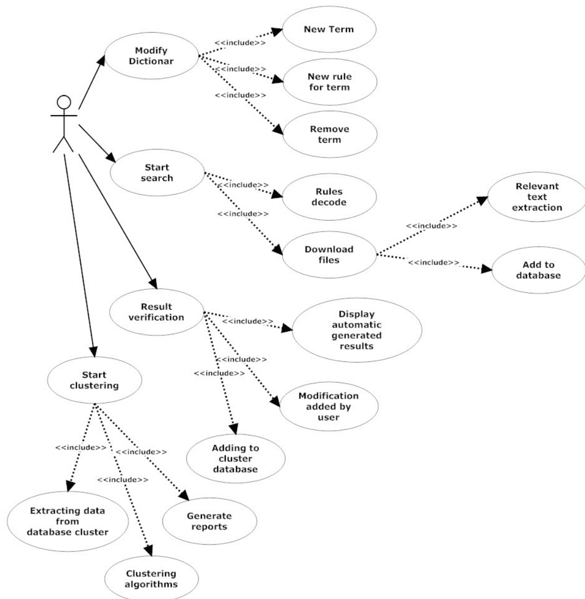
Fig. 4. IRS user use case diagram
