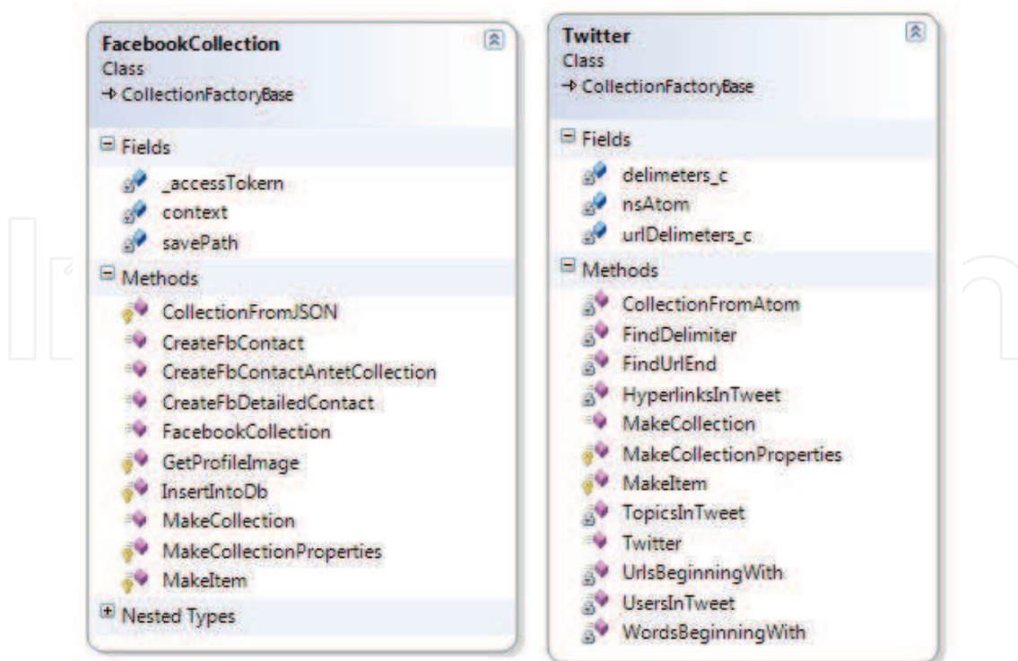
Fig. 2. The main classes used for connection with Facebook and Twitter
