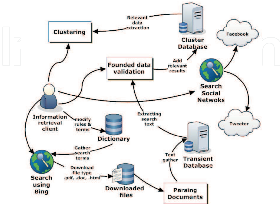
Fig. 1. The proposed IRS system structure
