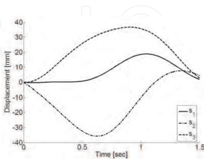
Fig. 28. Computed leg displacements of the waist module for the three legs
