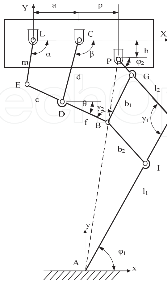
Fig. 2. A kinematic scheme of the single DOF Chebyshev-Pantograph leg mechanism
