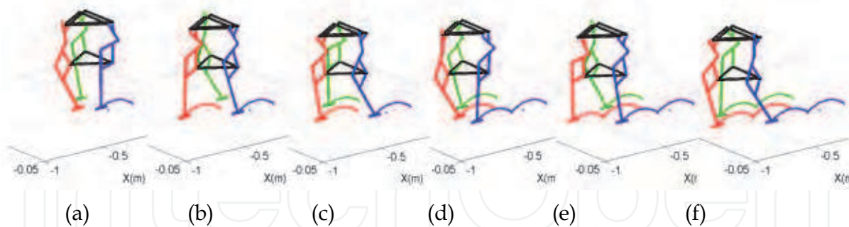
Fig. 14. Walking snapshots of the tripod walking robot as function of the input for leg motion: (a) \alpha_1=270 degs; (b) \alpha_1=90 degs; (c) \alpha_1=180 degs; (d) \alpha_1=270 degs; (e) \alpha_1=90 degs; (f) \alpha_1=180 degs
