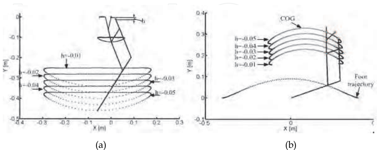
Fig. 10. A parametric study of the biped robot as function of parameter h in Fig. 2: (a) generated ovoid curves at point A; (b) trajectories of COG and foot point of swinging leg
