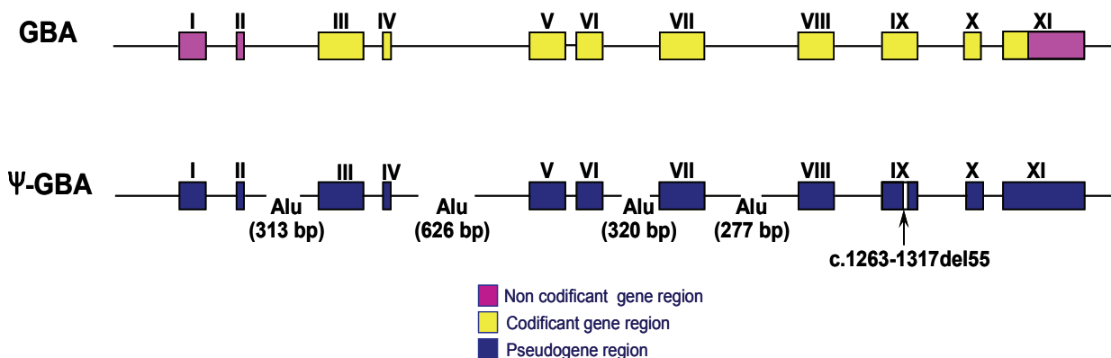
Fig. 4. Structure of glucocerebrosidase gene GBA and Pseudogene \Psi - GBA
