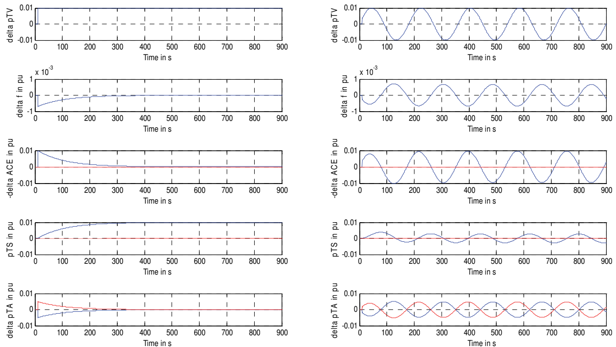
Fig. 7. Principle of operation of the secondary control if a step-shaped (left) and a sine-shaped (right) disturbance occurs
