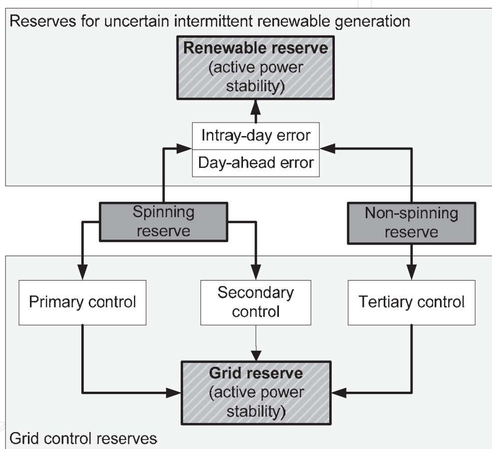
Fig. 10. Classes and types of different power reserves
