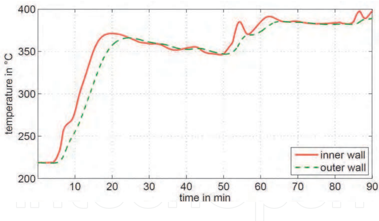
Fig. 16. Metal temperatures in the SH 2 outlet header
