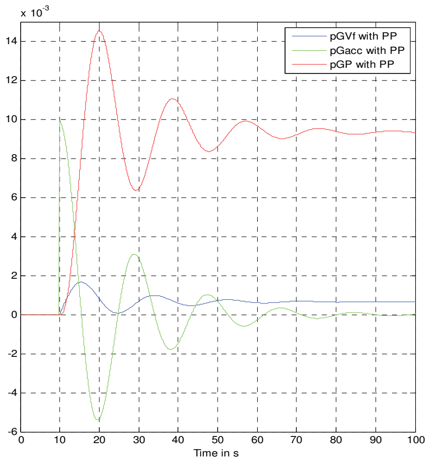
Fig. 4. Disturbance of the power balance covered by accelerating power, the consumer self-controlling effect and the primary control
