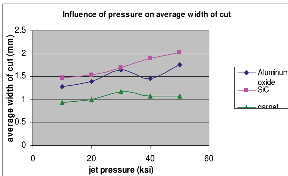
Fig. 21. Effect of pressure on width of cut
