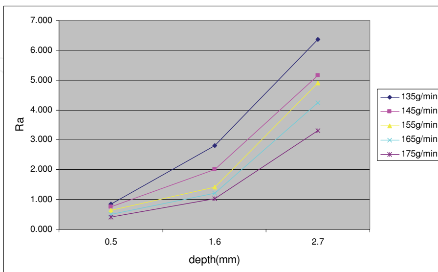
Fig. 11. Surface roughness at different depths from the top surface of carbide
