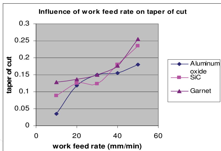
Fig. 17. Influence of feed rate on taper of cut
