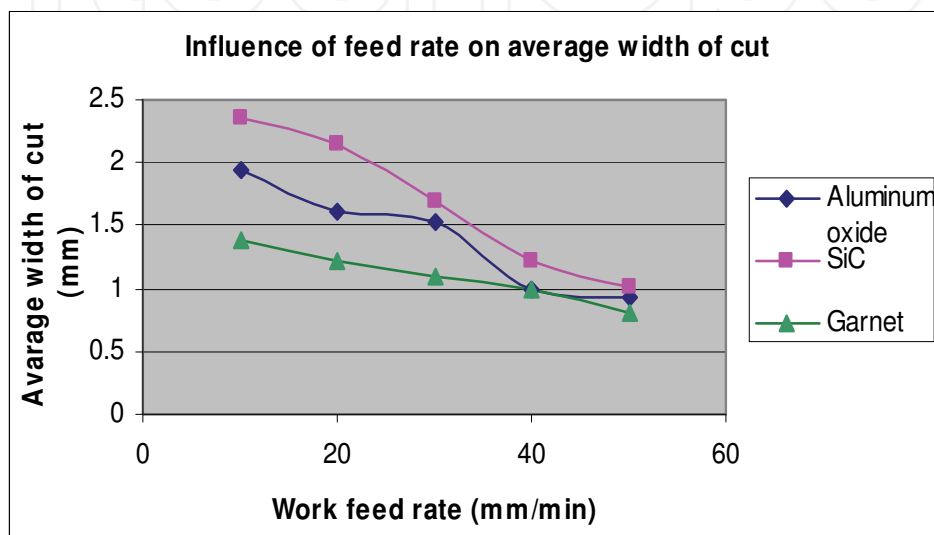
Fig. 20. Effect of feed on width of cut
