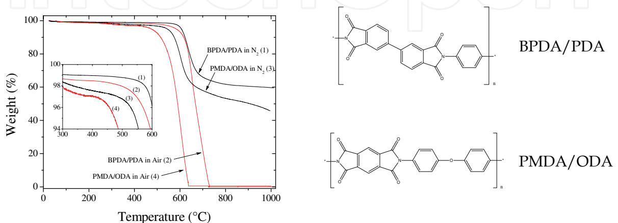
Fig. 2. Dynamical TGA of different structural PI films 2
