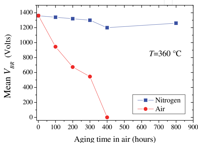
Fig. 15. Influence of the ambient atmosphere on the life time of the mean breakdown voltage of 4\text{ }\mu\text{m} -thick BPDA/PDA PI films at 360\text{ }^\circ\text{C}
