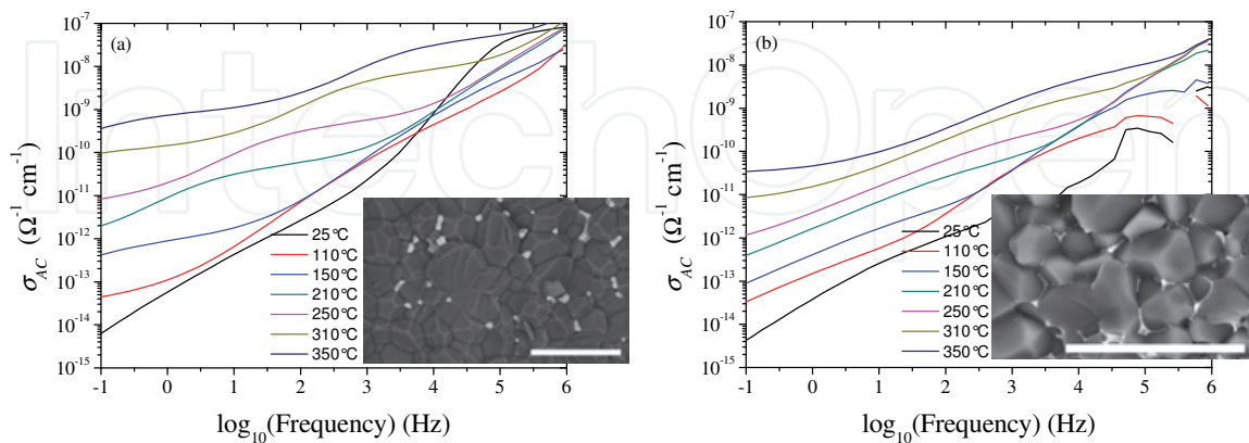
Fig. 8. Sintering process influence on the AC conductivity of 1800 °C-sintered AlN: (a) conventional sintering process and (b) SPS sintering process. Bar length: 10 \mu\text{m}
