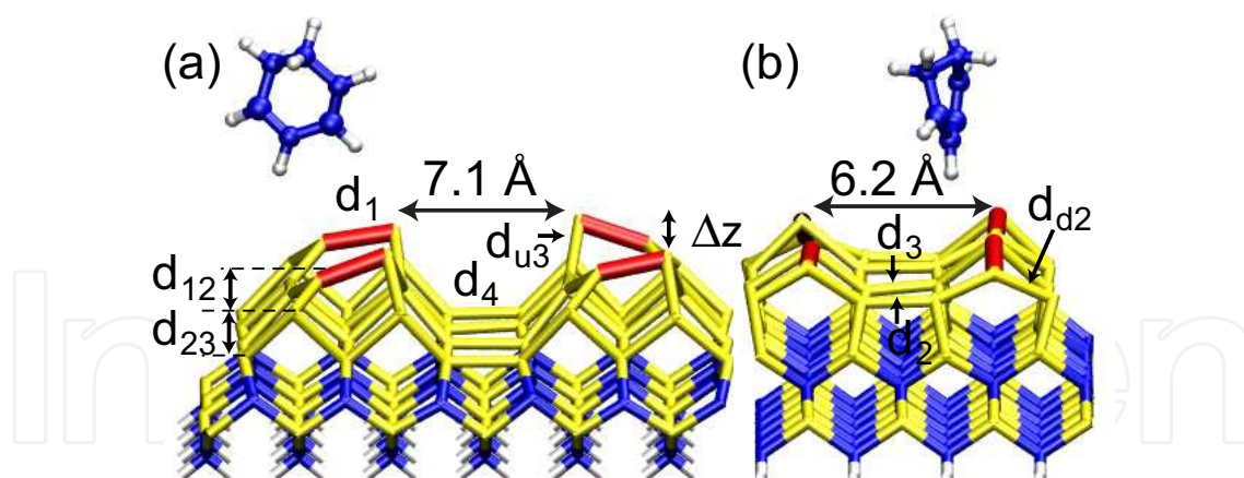
Fig. 1. View of 1,3-CHD + 3C-SiC(001)-3 \times 2 system (a) along dimer rows and (b) between dimers in a row. Si, C, H, and the top Si surface dimers are represented by yellow, blue, white, and red, respectively. The dimers are spaced farther apart by \sim 60\% along a dimer row and \sim 20\% across dimer rows relative to Si(100)-2 \times 1.
