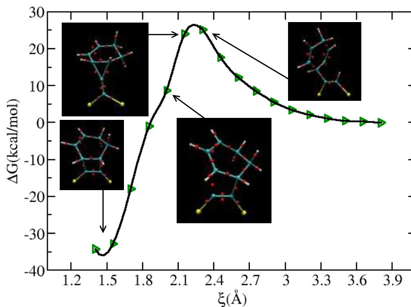
Fig. 9. Free energy profile for the formation of the [2+2] adduct between 1,3-cyclohexadiene and a C≡C dimer on the SiC-2×2 surface. Blue, white and yellow spheres represent C, H, and Si, respectively. Red spheres are the centers of maximally localized Wannier functions.
