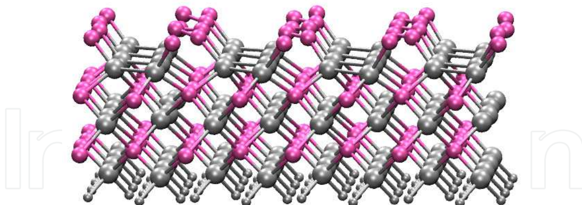
Fig. 5. Snapshot of the SiC-2×2 surface. Pink and grey spheres represent carbon and silicon atoms, respectively.
