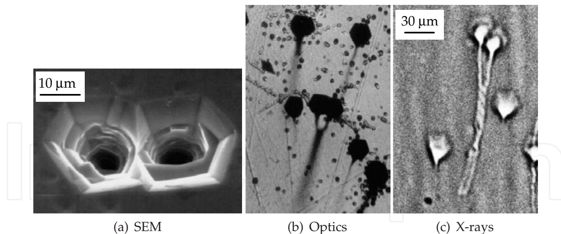
Fig. 4. (a) SEM image of a ramified micropipe; (b) transmission light microscopy image of the same micropipe; (c) SR phase-contrast image of another ramified configuration.
