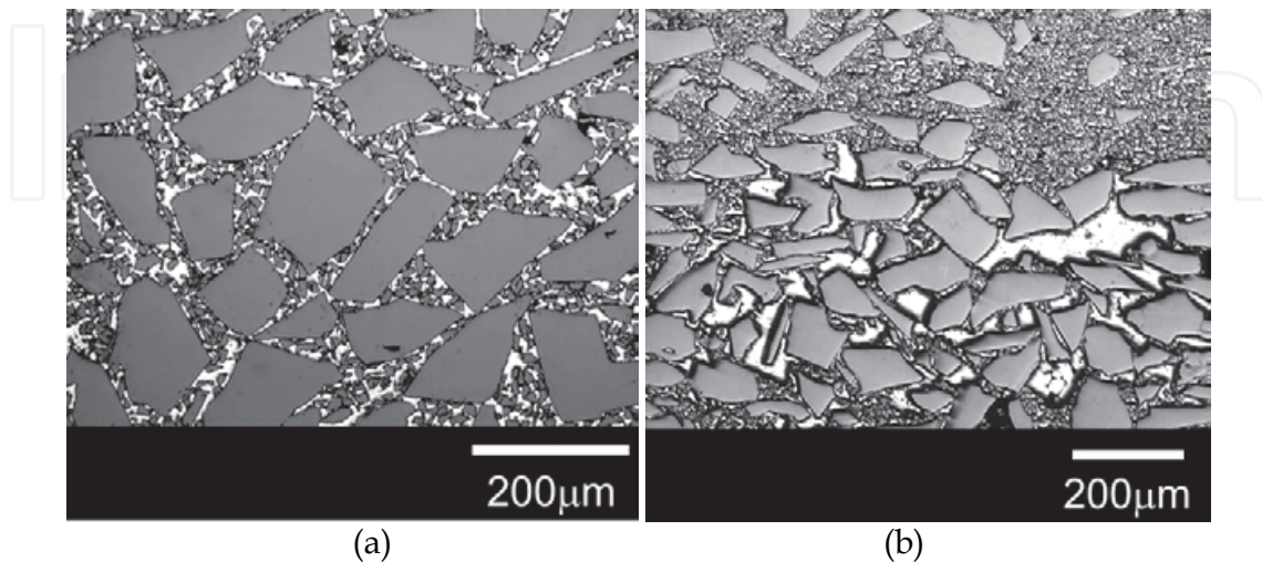
Fig. 6. Optical micrographs of cross sections of different samples of Al/SiC composites containing a mixture of SiC particles of two largely different sizes (17 \mu\text{m} and 170 \mu\text{m} ) in different proportions: (a) 67% coarse particles + 33% small particles; and (b) 75% coarse particles + 25% small particles, showing inhomogeneous filling
