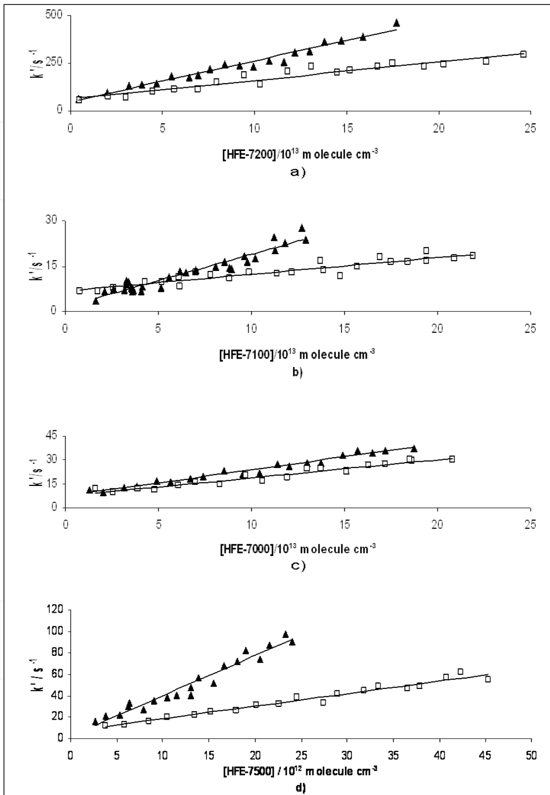
Fig. 3. Plots of the pseudo-first-order rate constants, k' , against segregated HFEs concentrations, at 1 Torr. a) HFE-7200+Cl = ( \blacktriangle ) 298 K and ( \square ) 234 K; b) HFE-7100+Cl = ( \blacktriangle ) 315 K and ( \square ) 263 K; c) HFE-7000+Cl = ( \blacktriangle ) 333 K and ( \square ) 266 K; d) HFE-7500+Cl = ( \blacktriangle ) 333 K and ( \square ) 253 K
