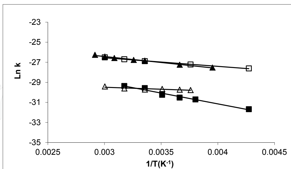
Fig. 4. Temperature dependence of the rate constant for: Cl+HFE-7200 ( \square ), Cl+HFE-7100 ( \blacksquare ), Cl+HFE-7000 ( \triangle ), and Cl+HFE-7500 ( \blacktriangle ) reactions at 1 Torr total pressure.
