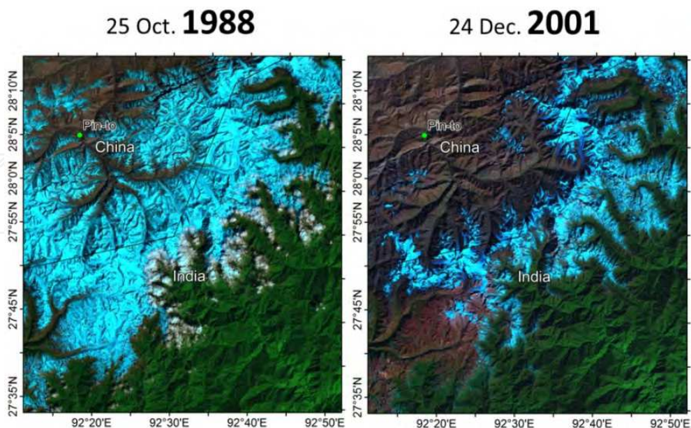
Fig. 2e. The Landsat images during year 1988 and 2001 show a sharp decline in the snow cover and enhanced melting of glaciers in the eastern Himalayas near the state of Arunachal Pradesh (India) and Tibet (China) border. ( Location 4, in Figure 1 ).
