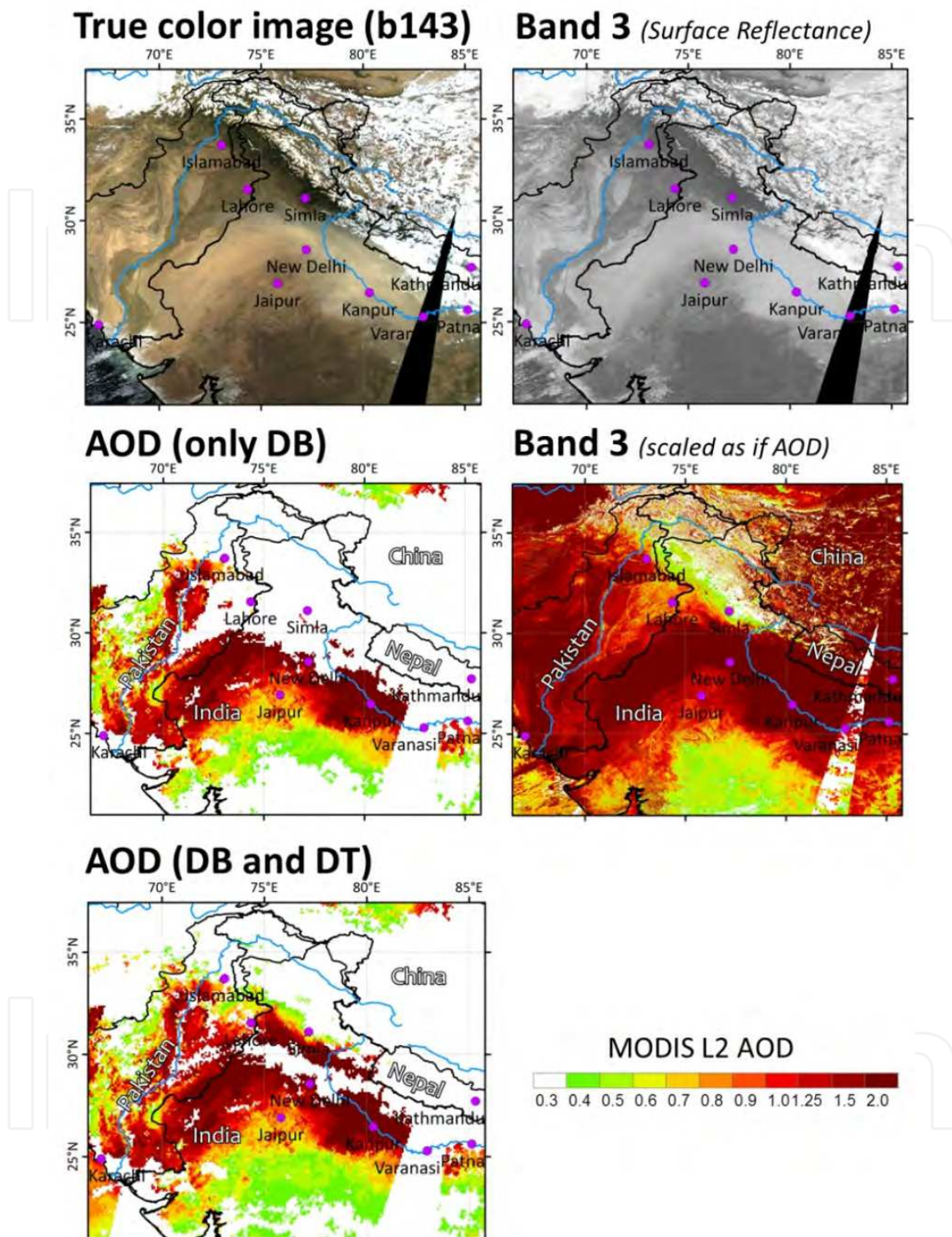
Fig. 7. The true color image (band combination: RGB: 1, 4, and 3) based on the MODIS Terra observations during a dust storm event on June 7, 2003. The dust affected region is prominent in the band 3 (blue band: 479 nm). The AOD (only DB) and AOD (combination of DB and DT) from level 2 Terra (collection 5.1) show quantitative aerosol loading due to the dust storm (marked as green to deep red color). The MODIS AOD like scaling using only MODIS band 3 (blue band) without any other filtering for cloud etc., illustrates its usefulness in deriving AOD over bright (arid) and low vegetative surfaces.
