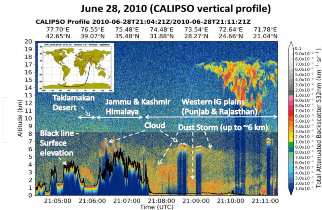
Fig. 14. The atmospheric profile (0-20 km) of a dust storm event as measured by the nighttime CALIPSO overpass over the western IG plain, and Himalayas during June 28, 2010 (at 2:35 to 2:41 am IST). The total attenuated backscatter (at 532 nm) shows the vertical structure of pre-dominantly dust aerosols up to ~6 km.
