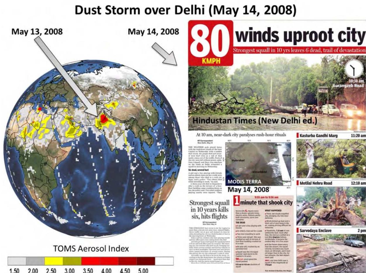
Fig. 6. The left panel shows arrival of the dust storm over Delhi region on May 13, 2008 using TOMS aerosol index (AI). The high values of TOMS AI (2.5-5) illustrate the aerosol loading associated with the dust storm. The right panel shows the after-effects of the dust storm over Delhi that was reported in several leading national newspapers (such as Hindustan Times, New Delhi edition on May 14, 2008).
