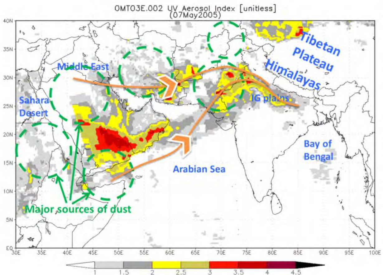
Fig. 4. The location of major sources of dust storms over the Indian sub-continent is marked as green broken circles (Prasad and Singh, 2007a). The two major pathways of dust storms, the sea route passing through the Arabian Sea and the land route, are marked by the orange line. The background shows Aura derived UV aerosol index during a dust storm event (May 7, 2005) that illustrates the transport of dust aerosols through the Arabian Sea before reaching the IG plains.
