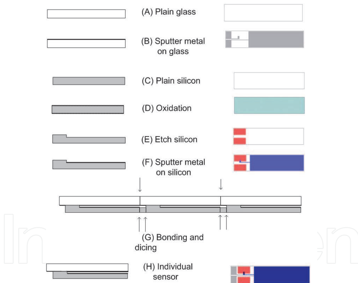
Fig. 3. Cantilever bending strain sensor fabrication process. Illustrations on the left are the side views and on the right are the top views. (a) Pyrex (Coring 7400) glass, (b) sputter of Au/Cr on glass as one electrode, (c) silicon substrate, (d) oxidation of the silicon as the etching mask, (e) etching silicon with KOH to create platforms for anodic bonding with glass, (f) sputter Au/Cr on silicon as the other electrode, (g) side view of partial dicing (arrows marks) after glass and silicon are anodically bonded, (h) the individual sensor after final separation, noting the gap between the two electrodes.
