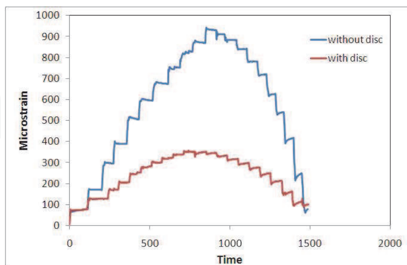
Fig. 13. Measured strains during excised spine testing.
