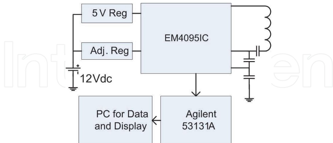
Fig. 7. The block diagram of the power reader.
