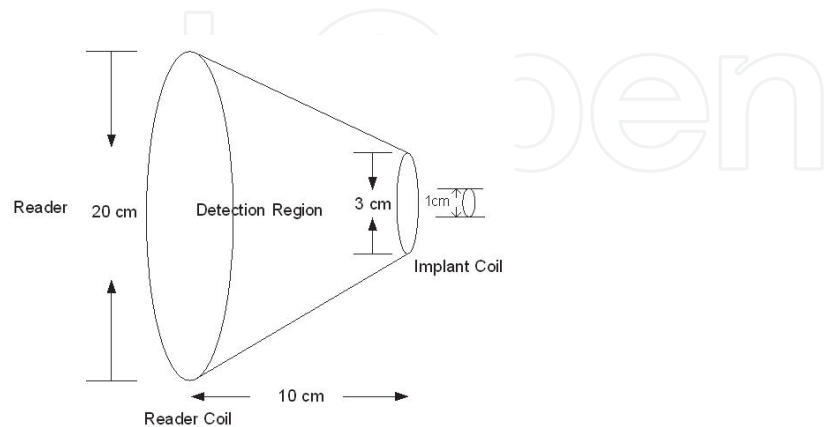
Fig. 8. The detection region is within the cone shape.
