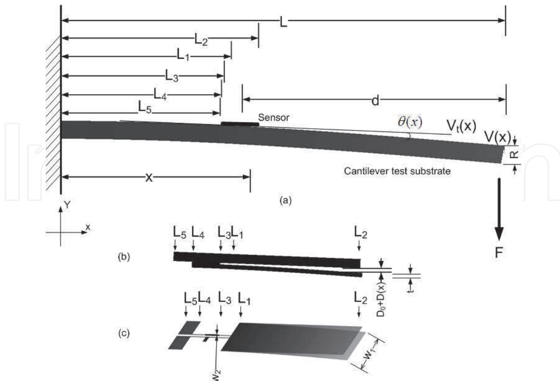
Fig. 2. The sensor on a substrate bar under bending. (b) The sensor's gap D_0 + D(x) , zoomed in from above, varies as a function of position x . (c) shows the respect metal coordinates on the cantilever substrate.
