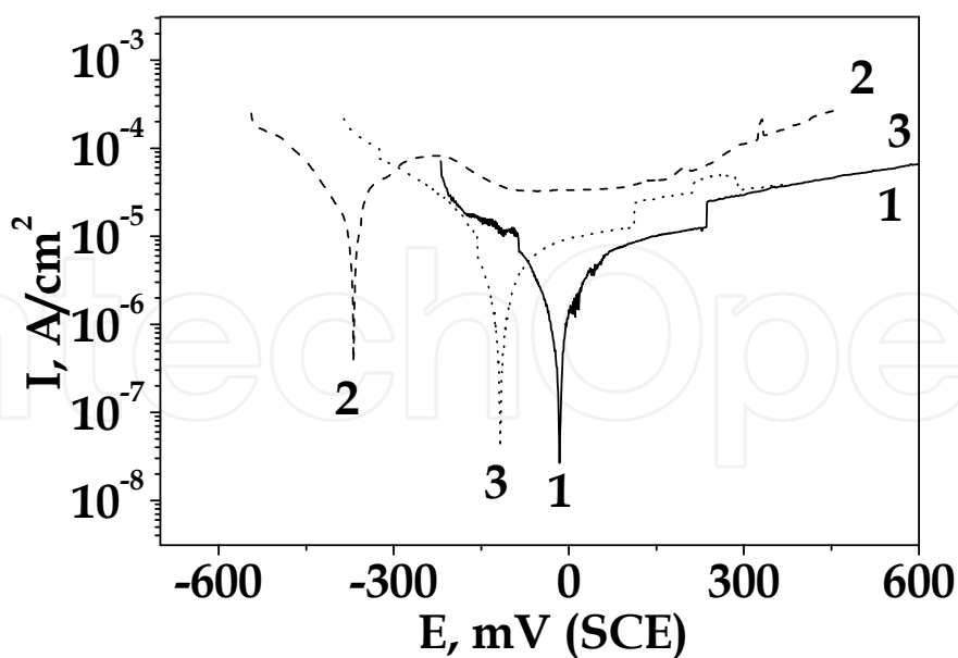
Fig. 6. PD polarization curves of HAS at 35 °C in: 1 - MCM; 2 - MCM with 300 \mu\text{g/L SO}_4^{2-} ; 3 - MCM with 300 \mu\text{g/L SO}_4^{2-} and 2 mg/L MEA.
