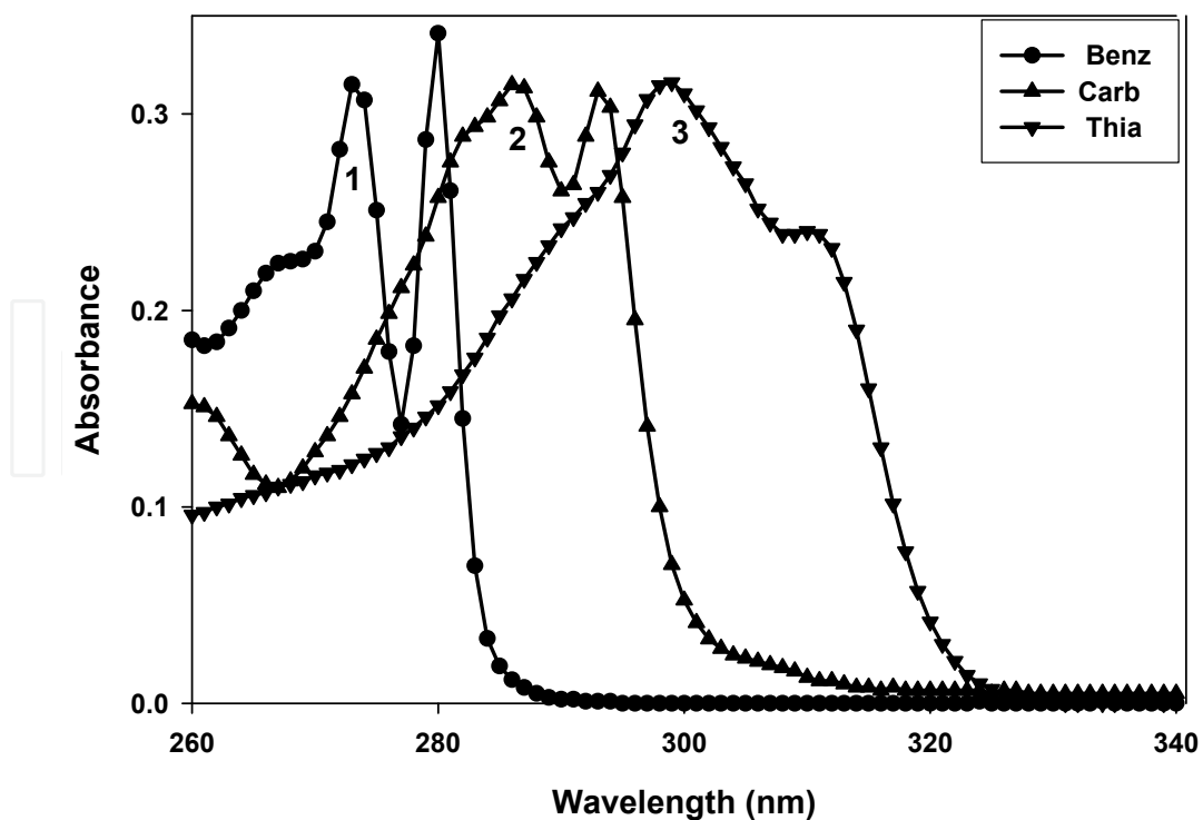
Fig. 2. UV absorption spectra of fresh samples of 1 \times 10^{-4} \text{M} solutions (1) benzimidazole, (2) carbendazime, (3) thiabendazole in acetonitrile solvent.
