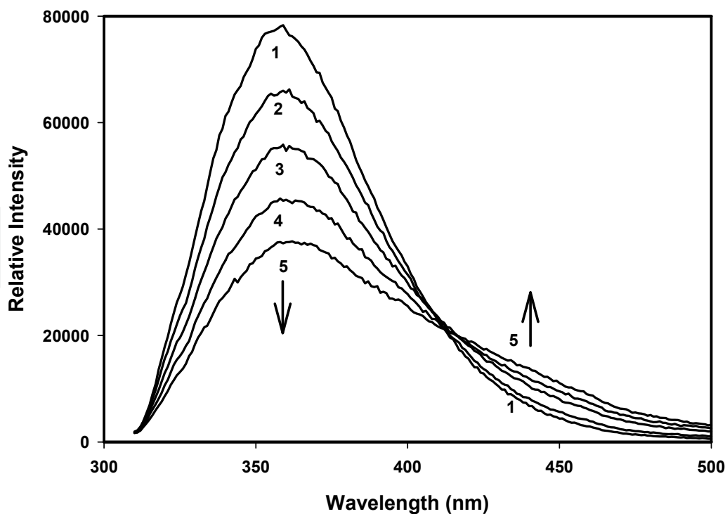
Fig. 12. Fluorescence spectra of fresh and photolyzed samples of 1.5 \times 10^{-4} \text{M} solutions of thiabendazole in acetonitrile solvent excited at 300 nm. (1) fresh, 2 5 min, (3) 10 min, (4) 15 min, (5) 20 min photolysis periods
