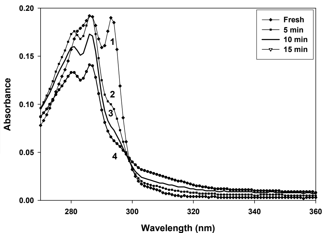
Fig. 8. UV absorption spectra of fresh and photolyzed samples of 0.5 \times 10^{-4} \text{M} solutions of carbendazim in acetonitrile solvent, (1) fresh, (2) 5 min, (3) 10 min, (4) 15 min photolysis periods.
