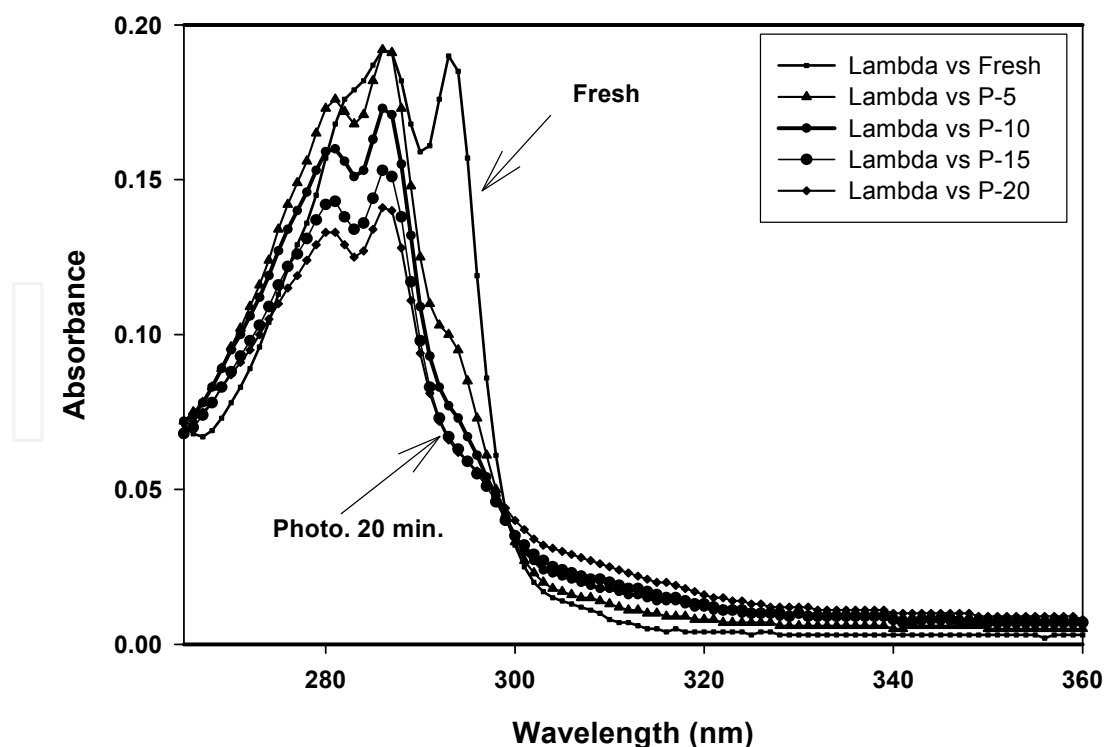
Fig. 11. UV absorption spectra of fresh and photolyzed samples of 1.5 \times 10^{-4} \text{M} solutions of thiabendazole in acetonitrile solvent.
