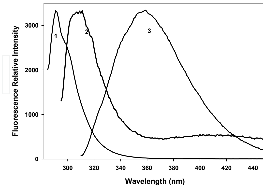
Fig. 3. Fluorescence spectra of fresh samples of 1 \times 10^{-4} M solutions (1) benzimidazole, (2) carbendazime, (3) thiabendazole in acetonitrile solvent. Excitation bands correspond to those obtained from the absorption maxima.
