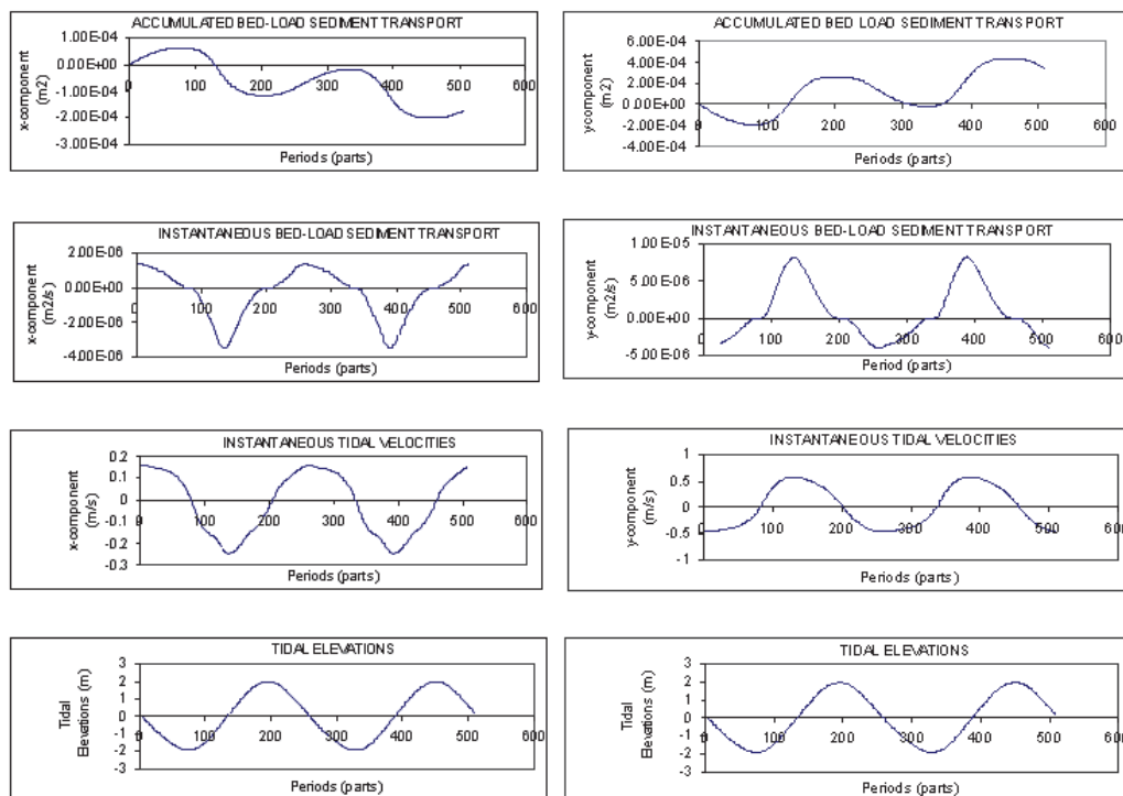
Fig. 5b. Sediment transport and hydrodynamic parameters obtained for two tidal periods at control point B.
