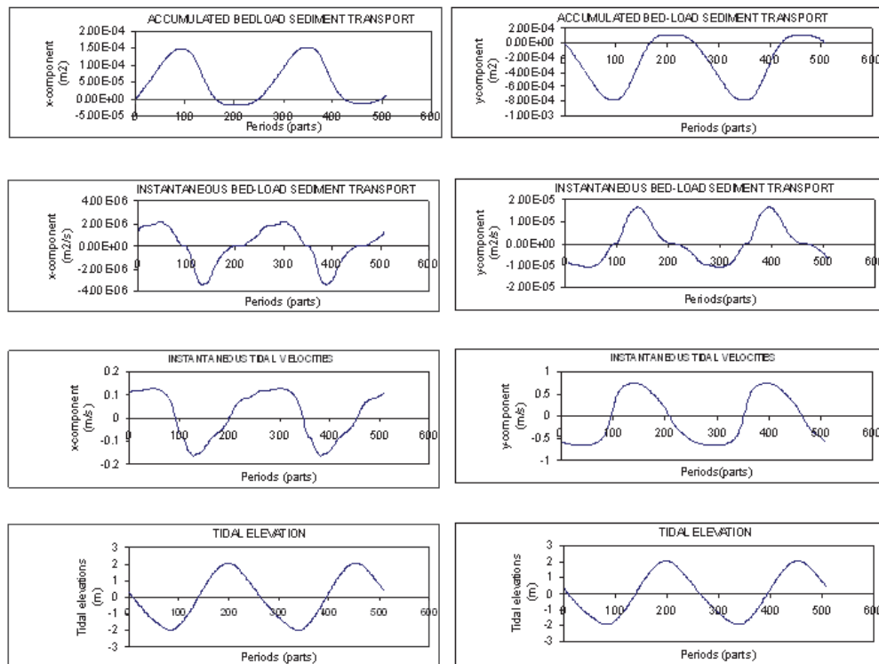
Fig. 5a. Sediment transport and hydrodynamic parameters obtained for two tidal periods at control point A.
