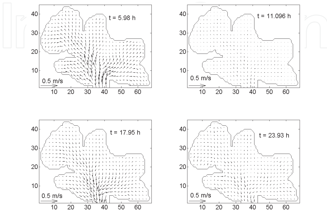
Fig. 8. Numerical modeling of currents produced by the soli-lunar declinational K_1 tide in the Yavaros Bay.
