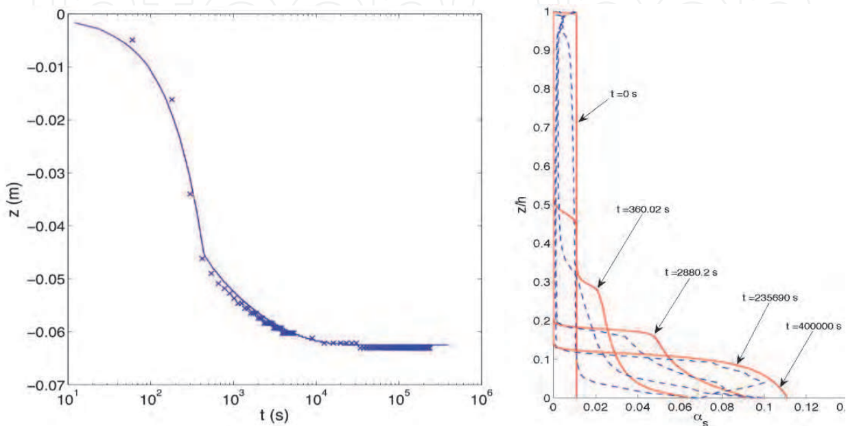
Fig. 9. Comparison of two-phase model results (—) with experiments (xxx) (Pham Van Bang, 2007) for initial concentrations \alpha_s^0=1.2\% : a) Settling curves: time evolution of the mud-clear water interface position and b) solid volume fraction profiles.
