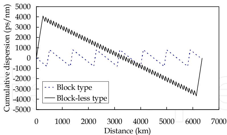
Fig. 4. Dispersion maps of the simulated systems
