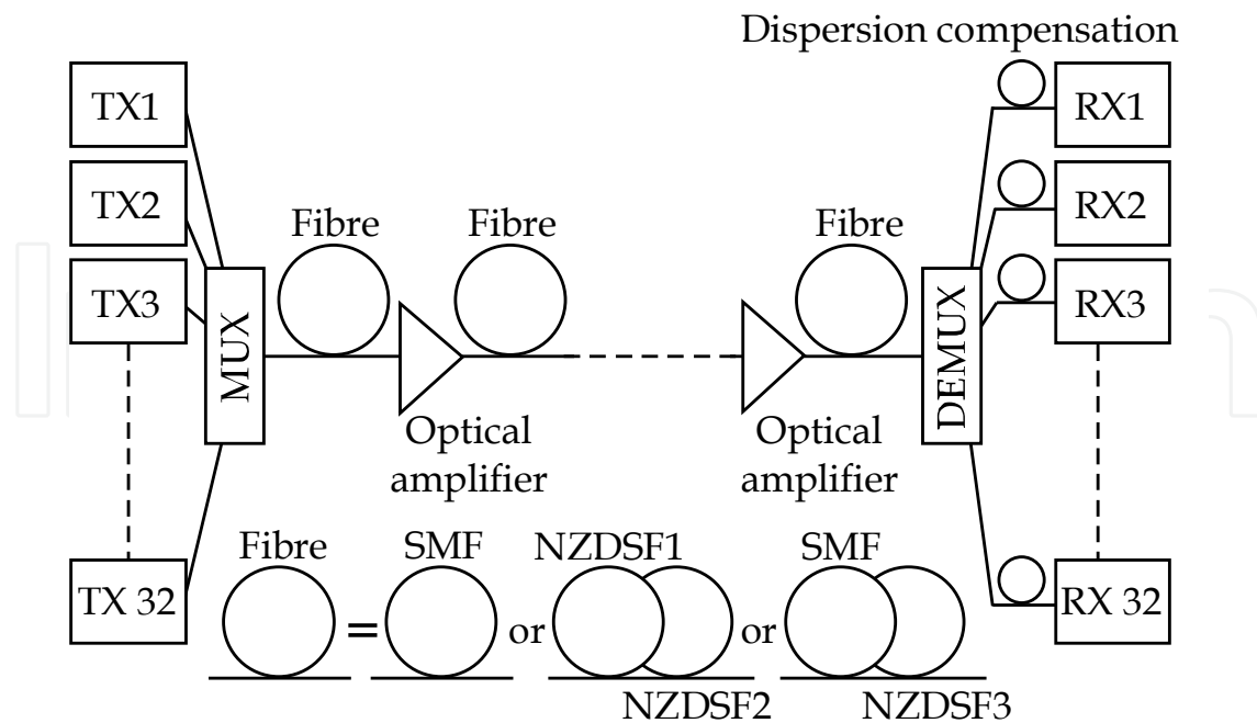
Fig. 3. A schematic diagram of the simulation model
