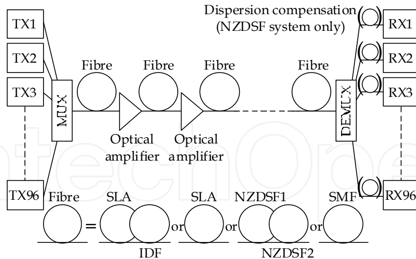
Fig. 12. A schematic diagram of the simulation model
