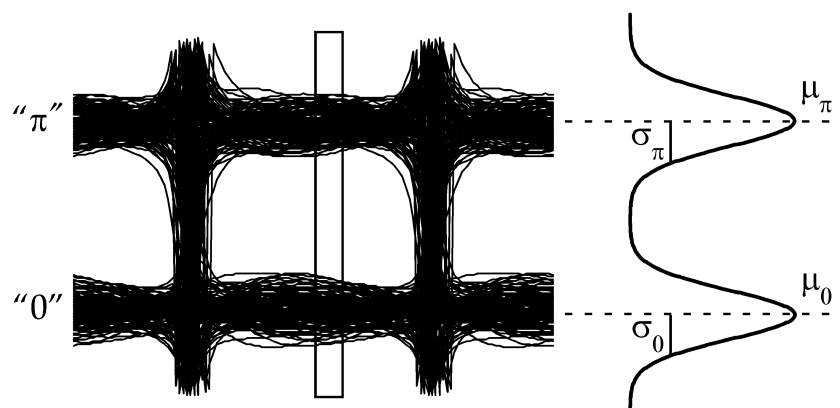
Fig. 2. Relationship of parameters and phase eye diagram
