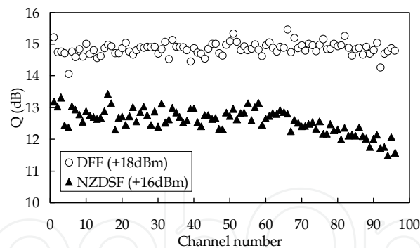
Fig. 16. Transmission performance of 96 channels with the optimum repeater output power
