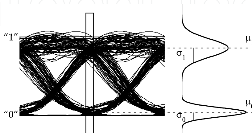
Fig. 1. Relationship of parameters and intensity eye diagram
