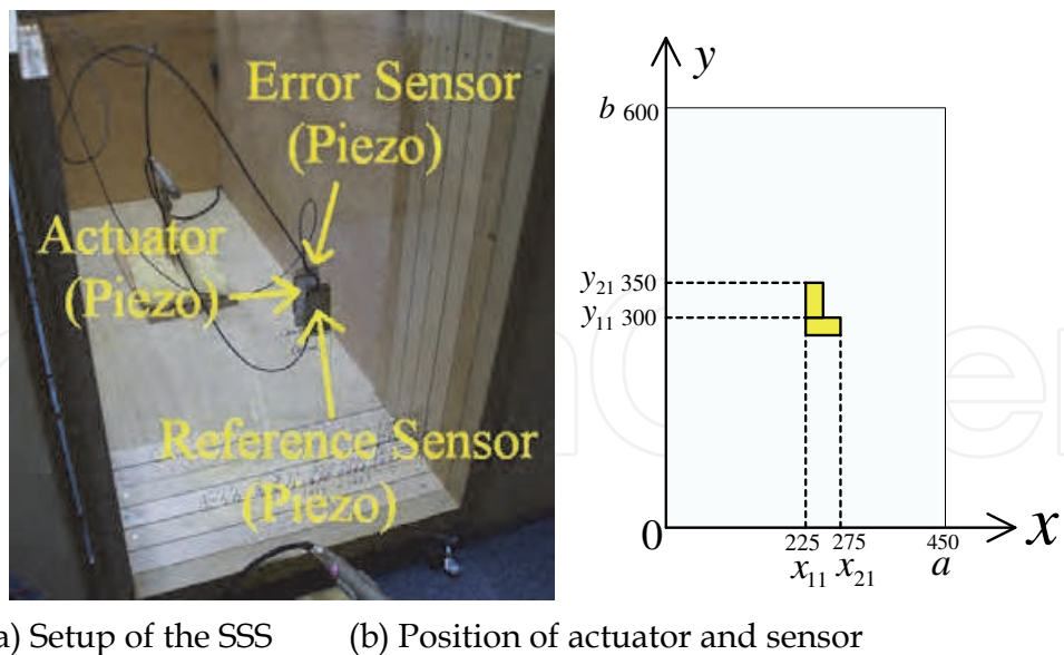
Fig. 1. Structure of the considered Sound Selection System
