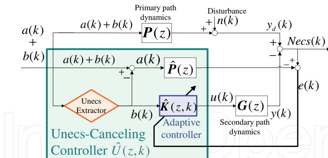
Fig. 5. Schematic diagram of the Unecs-Canceling Controller (One of the SSC)
