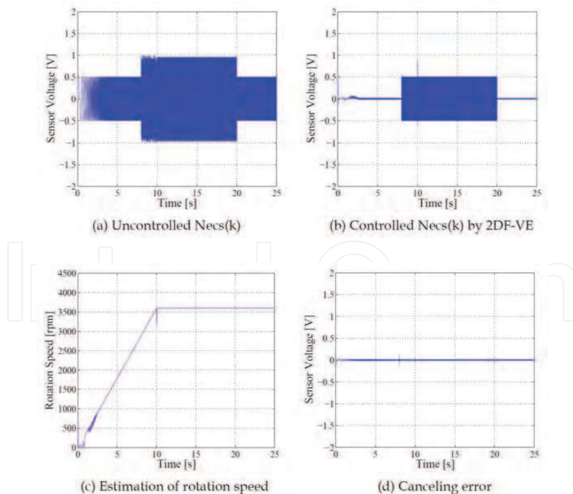
Fig. 13. Simulation results of Unecs-Canceling Controller
