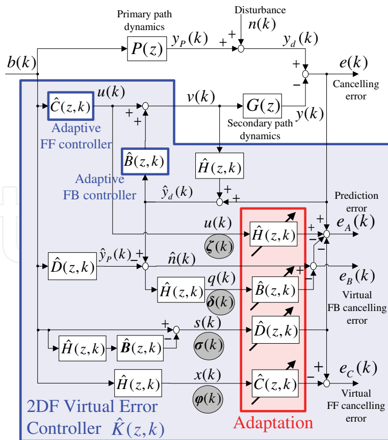
Fig. 10. Block diagram of the 2-degree-of-freedom Virtual Error controller
