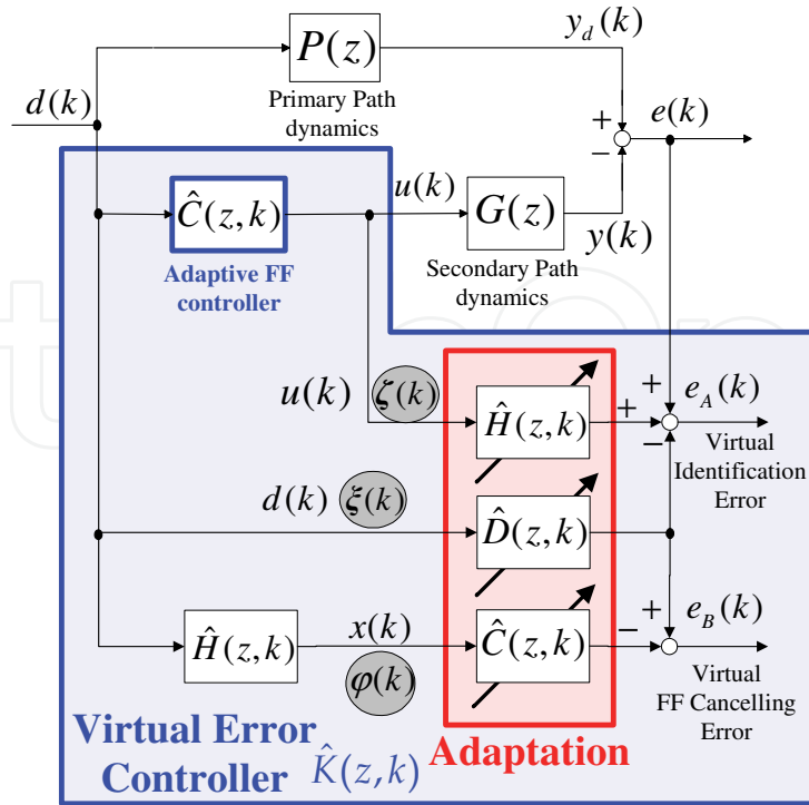
Fig. 9. Block diagram of the Virtual Error controller
