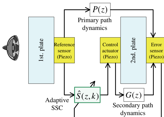
Fig. 2. Schematic diagram of the considered SSS
