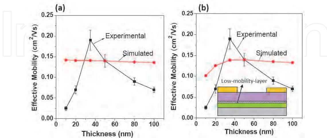
Fig. 8. (a) A comparison of the mobility values for the experimental and the simulated devices and (b) between experimental and simulated devices on incorporating the low-mobility-layer as a function of pentacene thickness. (Reprinted from Organic Electronics , Vol. 11, D. Gupta, Y. Hong, "Understanding the effect of semiconductor thickness on device characteristics in organic thin film transistors by way of two dimensional simulations", pp. 127-136, 2010, with permission from Elsevier)
