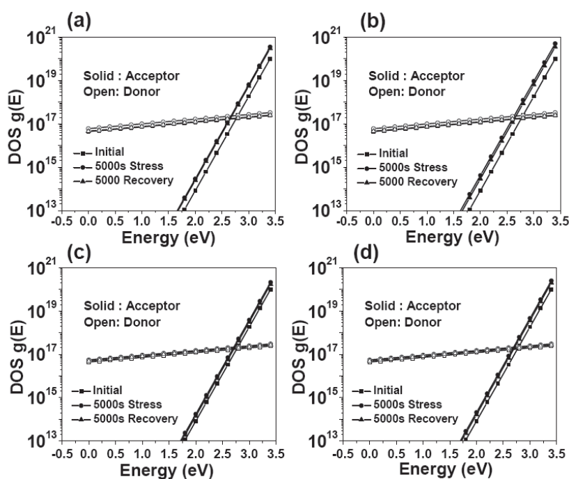
Fig. 12. Variation in density of states (DOS) during stress and recovery period for stress values of (a) 20 V of gate bias, (b) 50 V of gate bias and (c) 5 \times 10^{-6} A of drain current and (d) 3 \times 10^{-5} A of drain current.
