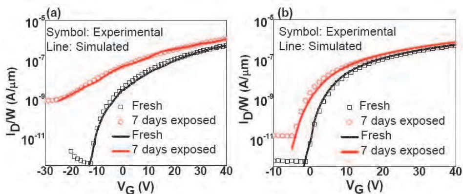
Fig. 13. Comparison of simulated and experimental transfer curves for (a) undoped and (b) 25% Li- doped ZnO TFTs in fresh state and after 7 days of air exposure at drain voltage of 40 V.
