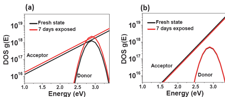
Fig. 14. The obtained density of states (DOS) distribution in the fresh state and after 7 days of air exposure for (a) undoped and (b) 25% Li- doped ZnO TFTs
