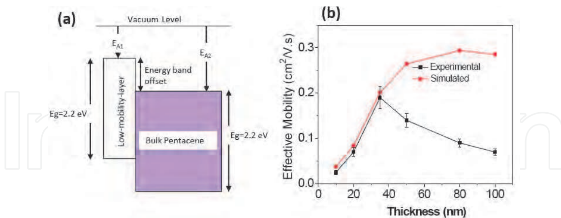
Fig. 9. (a) Schematic diagram of the energy levels in the low mobility layer and bulk of the pentacene film (b) Comparison of experimental and simulated mobility value as a function of pentacene thickness. The mobility of the low-mobility-layer is 1 \times 10^{-4} cm 2 /Vs and bulk mobility is 1.3 cm 2 /Vs. The energy band offset value is 0.11 eV. (Reprinted from Organic Electronics , Vol. 11, D. Gupta, Y. Hong, "Understanding the effect of semiconductor thickness on device characteristics in organic thin film transistors by way of two dimensional simulations", pp. 127-136, 2010, with permission from Elsevier)
