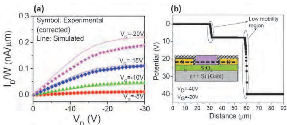
Fig. 6. (a) Comparison of the experimental (gate leakage and contact corrected) and the simulated output curves. The mobility of the low-mobility-region is 1.5 \times 10^{-4} \text{ cm}^2/\text{Vs} and bulk mobility of pentacene is 0.14 \text{ cm}^2/\text{Vs} . (b) Surface potential profile 1 nm above the dielectric surface (source, drain and channel lie between 0\text{-}30 \mu\text{m} , 60\text{-}90 \mu\text{m} and 30\text{-}60 \mu\text{m} , respectively). (Reprinted from Organic Electronics , Vol. 10, No. 1, D. Gupta, M.Katiyar, Deepak, "An analysis of difference in device behavior of top and bottom contact devices using device simulation", pp. 775-784, 2009, with permission from Elsevier)
