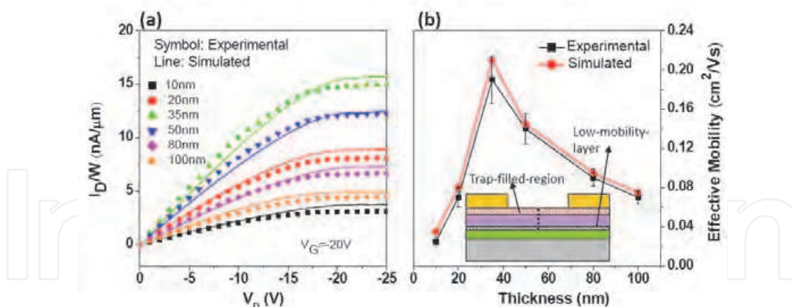
Fig. 10. A comparison of simulated and experimental (a) output curves and (b) mobility value as a function of pentacene thickness. The mobility of the low-mobility-layer and bulk pentacene is taken as 1 \times 10^{-4} \text{ cm}^2/\text{Vs} and 1.3 \text{ cm}^2/\text{Vs} , respectively. The energy band offset value is 0.11 \text{ eV} . The trap concentration is taken as 4 \times 10^{16} \text{ cm}^{-3} for 50 \text{ nm} thick film and 6 \times 10^{16} \text{ cm}^{-3} for 80 and 100 \text{ nm} thick films, respectively. (Reprinted from Organic Electronics , Vol. 11, D. Gupta, Y. Hong, "Understanding the effect of semiconductor thickness on device characteristics in organic thin film transistors by way of two dimensional simulations", pp. 127-136, 2010, with permission from Elsevier)
