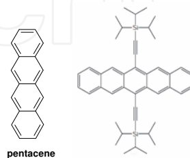
Fig. 1. Chemical structure of (a) pentacene and (b) TIPS- pentacene molecule.
