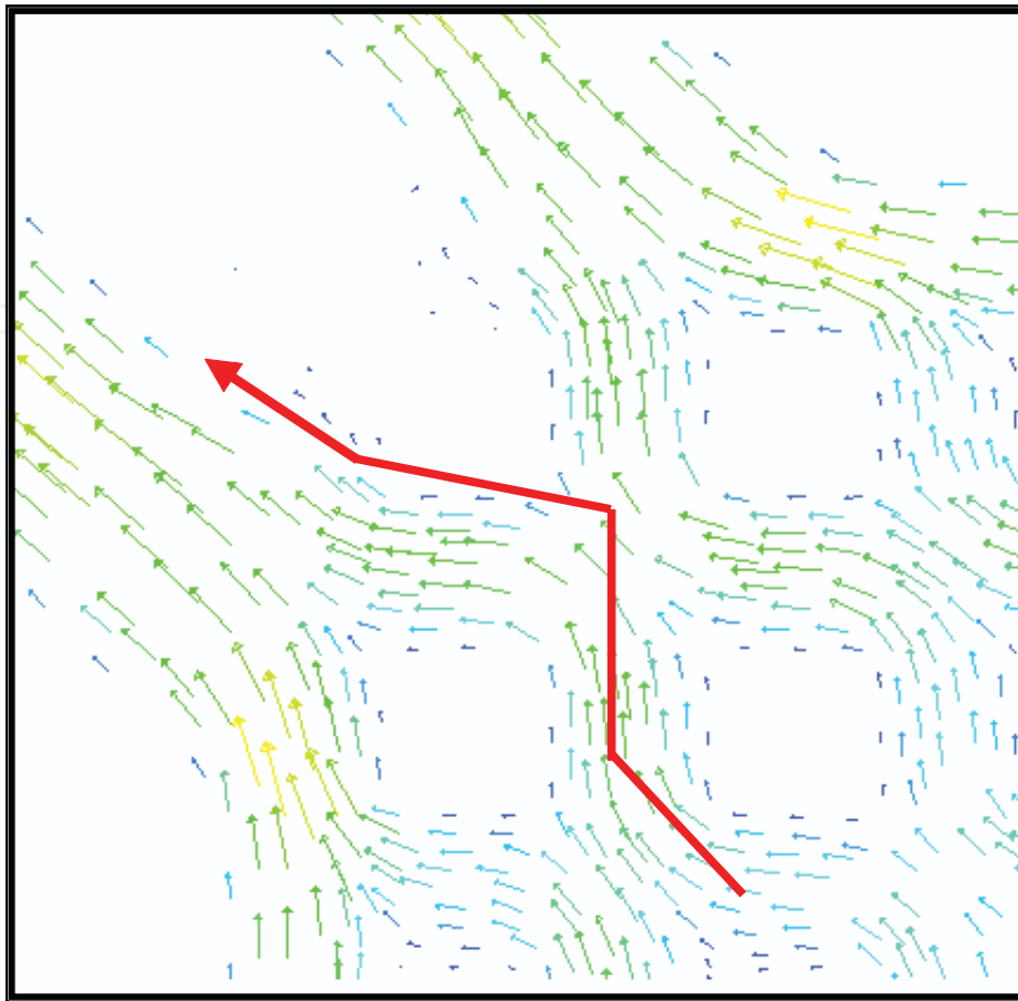
Fig. 5. Flow of cross strip in outlet
