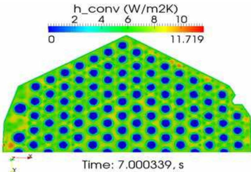
Fig. 23. Bottom Plate Heat Transfer Coefficient
