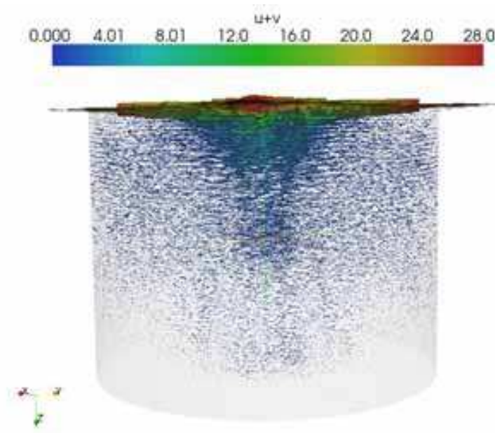
Fig. 7. Fast Decay of the Azimuthal Velocity
