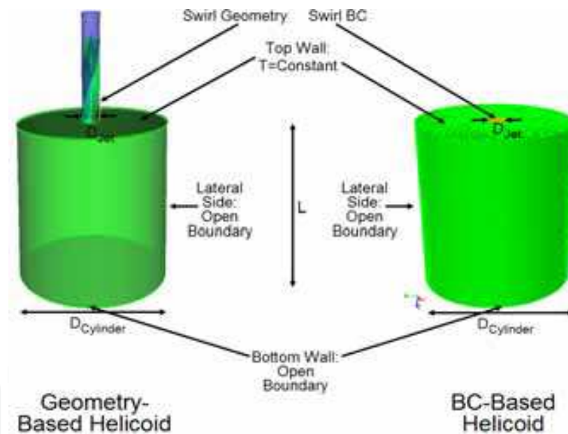
Fig. 4. Comparison of Geometric and BC Swirl Models
