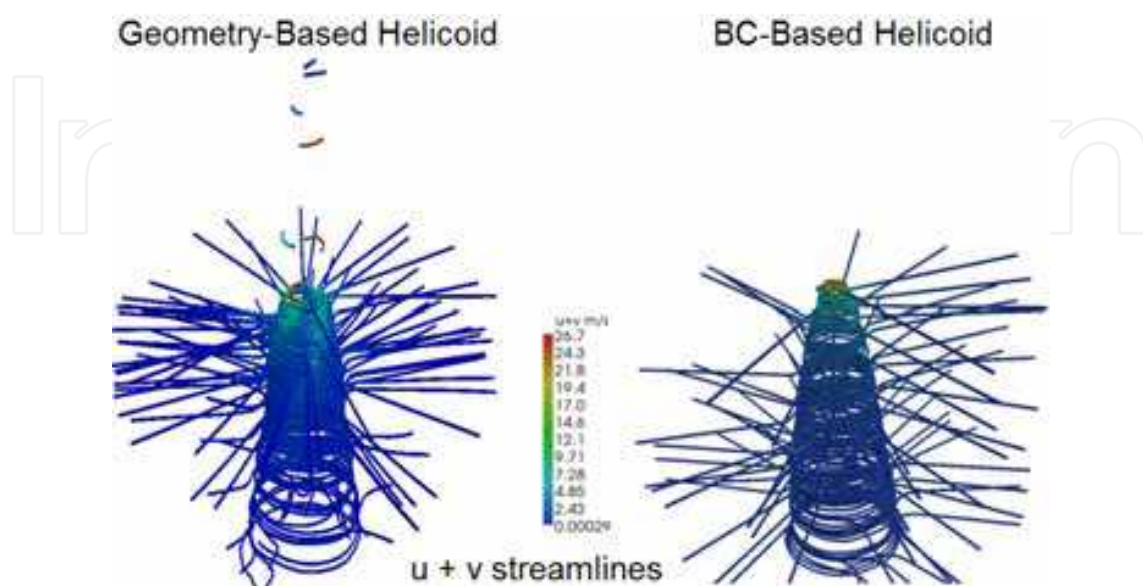
Fig. 6. Comparison of the Geometric and BC Swirl Models: Azimuthal Velocity Streamlines
