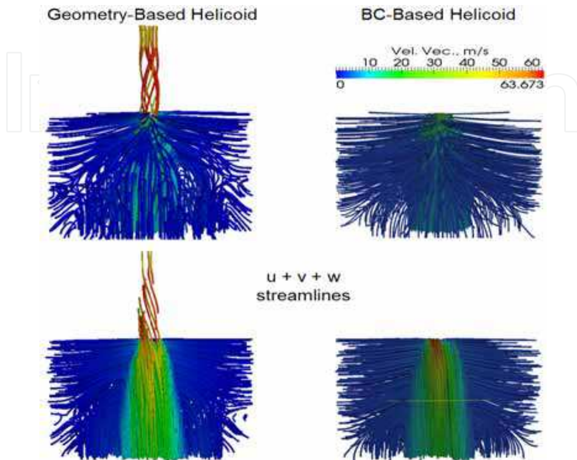
Fig. 5. Comparison of the Geometric and BC Swirl Models: U + V + W Streamlines
