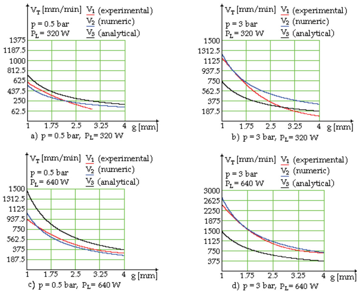
Fig. 6. Processing speed variation
