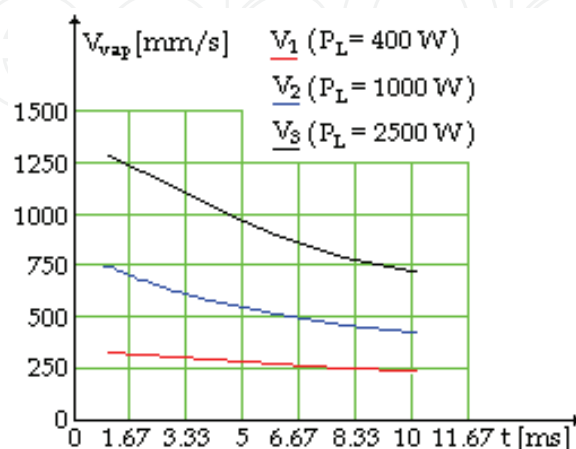
Fig. 5. The vaporization speed variation vs. processing time
