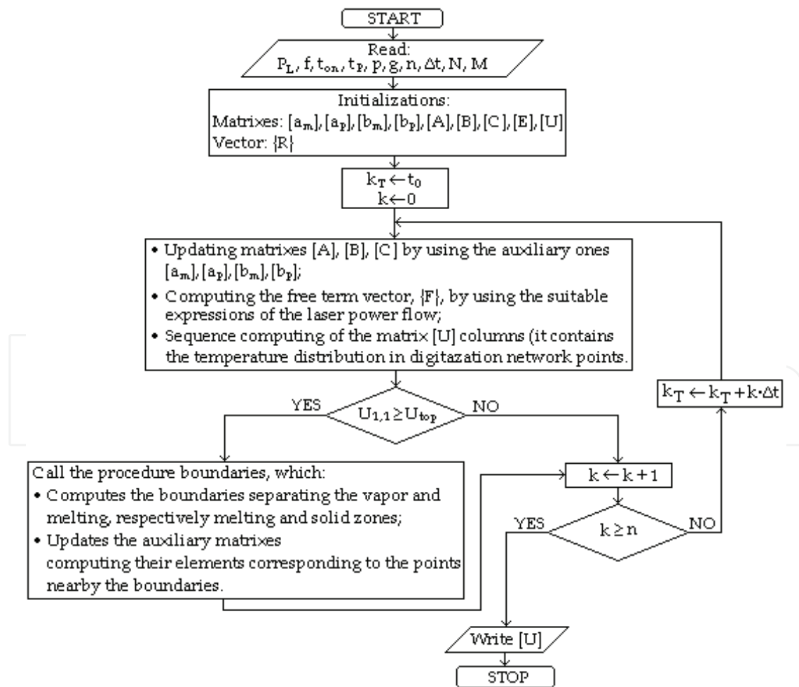
Fig. 2. Logical diagram of the function computing the temperature distribution in material
