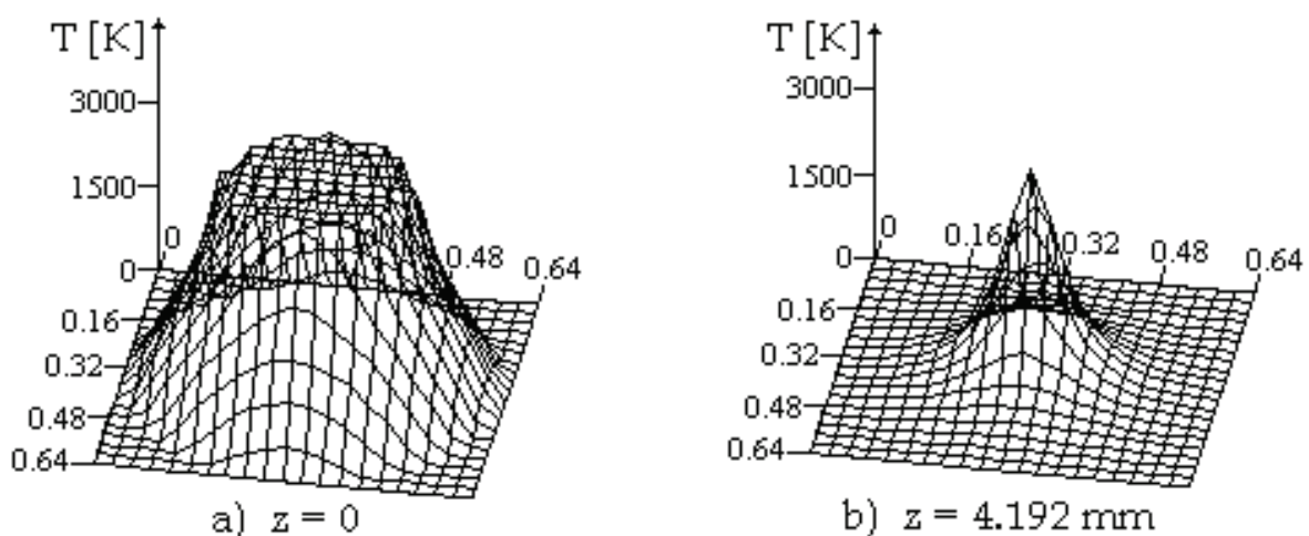
Fig. 3. Temperature distribution, P_L = 1\text{kW} , t = 10\text{ms}
