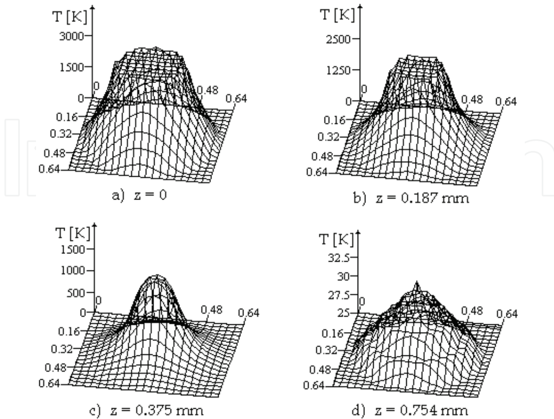
Fig. 4. Temperature distribution, P_L = 400 W, t = 1 ms
