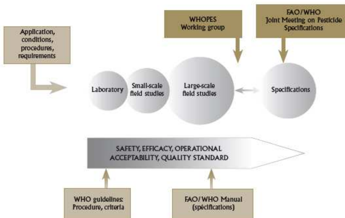
Fig. 4. World Health Organization Pesticide Evaluation Scheme (WHOPES).
