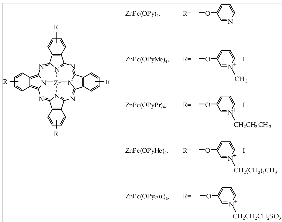
Fig. 1. Chemical structure of Zn(II)-phthalocyanine with pyridyloxy substituents with increasing hydrocarbon chain to N-atom
