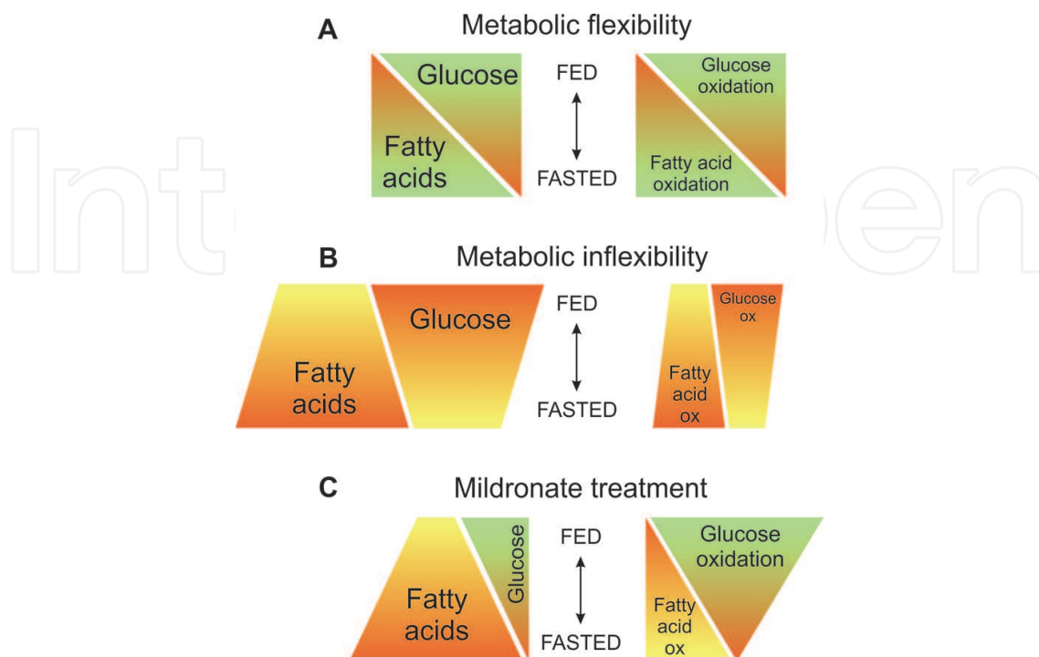
Fig. 5. Metabolic flexibility, inflexibility and mildronate treatment induced protection against lipid overload.
