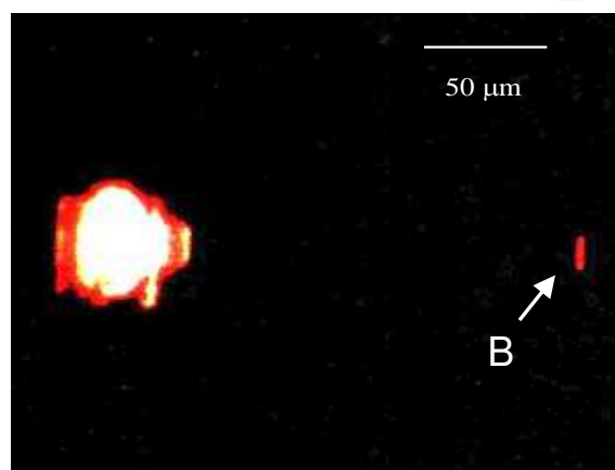
Fig. 13. Photomicrographs of a CMOS opto-coupler arrangement consisting of a CMOS Av-based light-emitting source, an optically waveguide and a CMOS lateral incident photo-detector. (a) shows a bright field photo-micrograph of the arrangement, and (b) shows the optical performance as observed under dark field conditions (Snyman et al, 2000, 2004).
