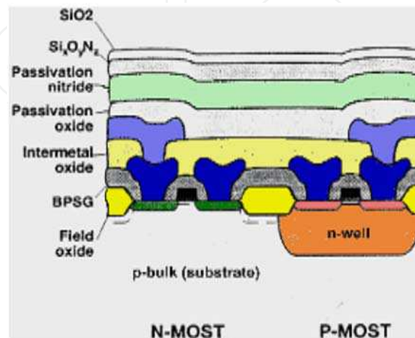
Fig. 1. Schematic diagram displaying a typical structure used in field oxide based CMOS integrated circuit technology. Layers that are optically transparent below 1 \mu\text{m} are shown in yellow, green and grey . Bright yellow: Native silicon dioxide; Yellow: intermetallic oxide; White: Passivation oxide ; Green: Silicon nitride.
