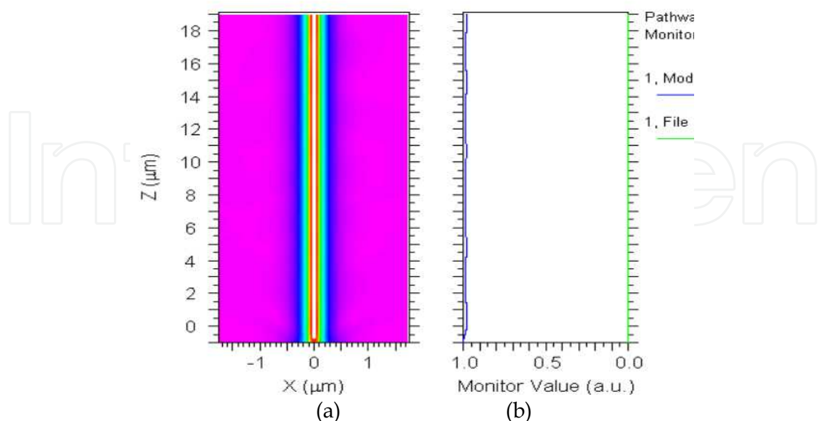
Fig. 11. (a) and (b): Advanced simulation of the electrical field propagation in a silicon nitride layer within CMOS integrated circuitry. Single mode propagation is demonstrated at 750 \text{ nm} over a distance of 20 \mu\text{m} for a 0.2 \mu\text{m} wide silicon nitride waveguide, embedded in \text{SiO}_2 .
