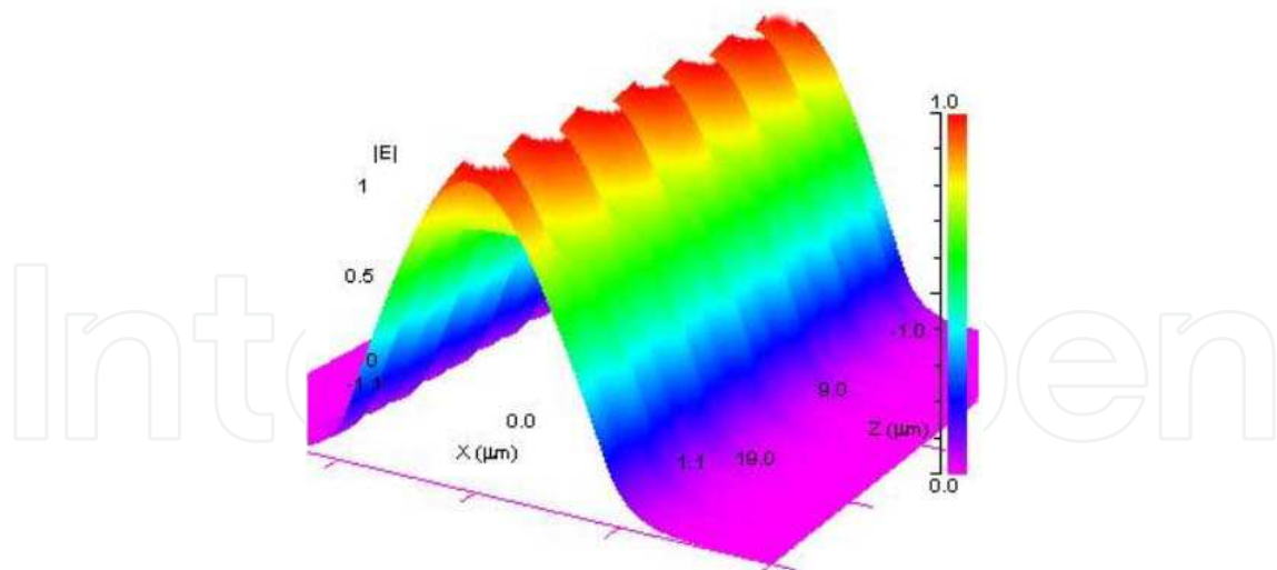
Fig. 10. Advanced optical simulation of the electrical field propagation in a 0.6 \mu\text{m} wide silicon nitride layer embedded in \text{SiO}_2 in CMOS integrated circuitry. Multimode optical propagation at 750 \text{ nm} is demonstrated over 20 \mu\text{m} with a loss of less than 1 \text{ dB cm}^{-1} .
