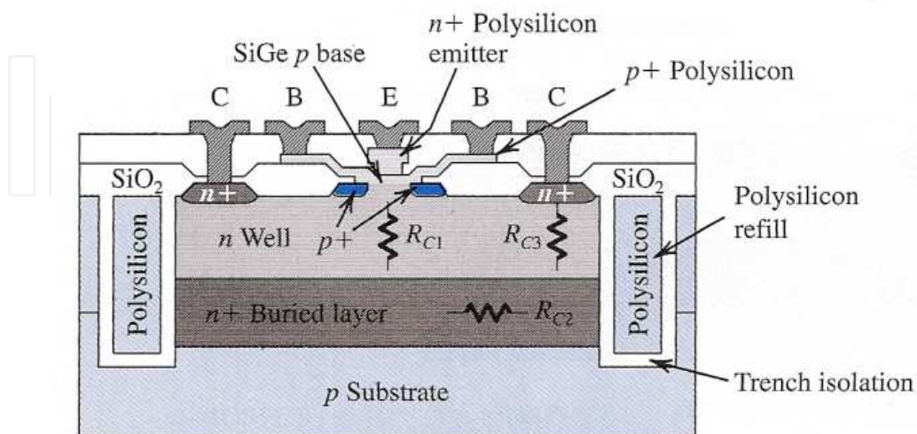
Fig. 4. Components and structural layout of the latest CMOS processes utilising isolation trench based technology (Sedra, 2004).
