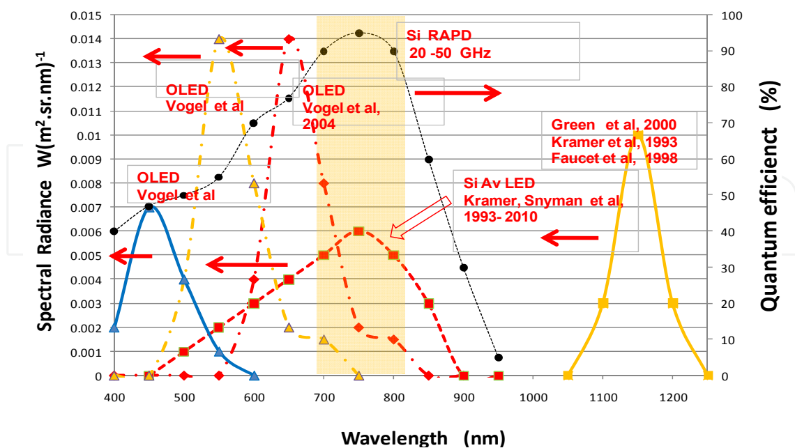
Fig. 6. Spectral radiance characteristics of Organic Light Emitting Devices (OLEDs and Si avalanche-based light emitting device (Si Av LED), and comparison with the spectral detection range of reach through avalanche detector (RAPD) devices.
