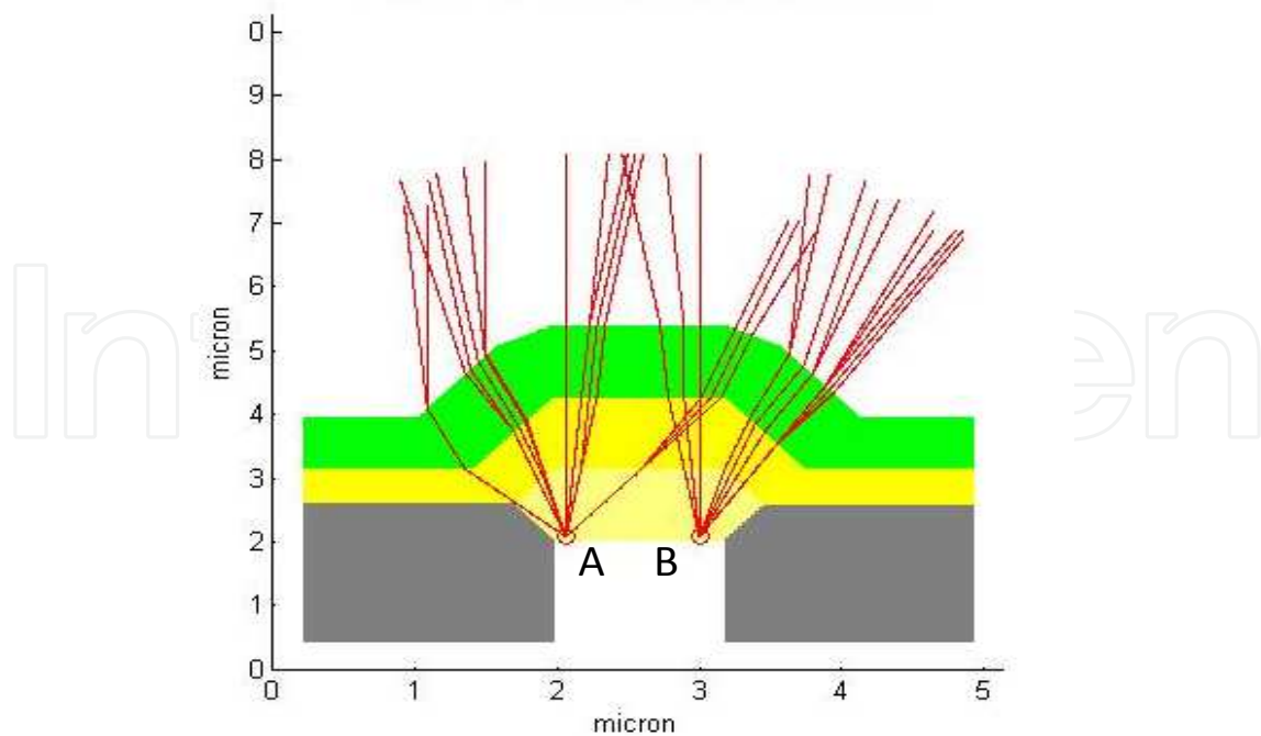
Fig. 2. Optical propagation phenomenon at 750nm in CMOS over layers using simple ray tracing techniques. The layer color indexing is the same as in Fig.1.
