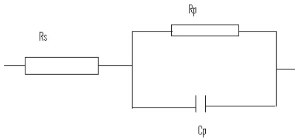
Fig. 12. Deducing equivalent circuit from impedance plots.
