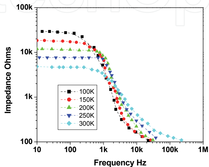
Fig. 14b. Impedance spectra of ITO/PEDOT:PSS/MEH:PPV/LiF/Al.
