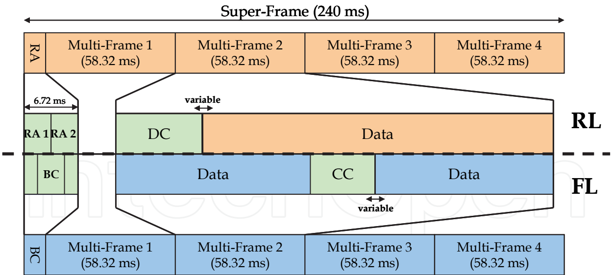
Fig. 11. Super-Frame Structure.
