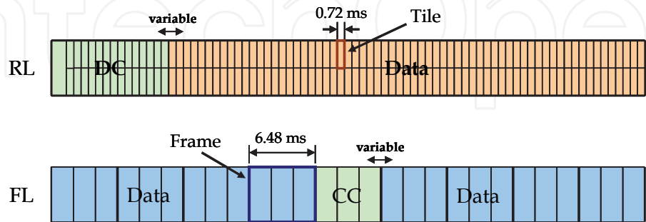
Fig. 10. Multi-Frame structures.
