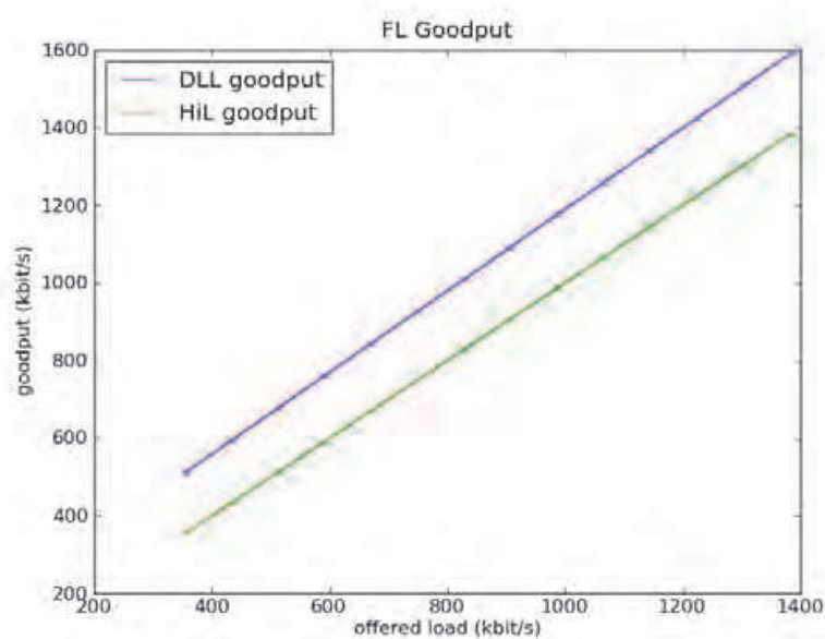
Fig. 22. FL goodput - scenario LOAD.
