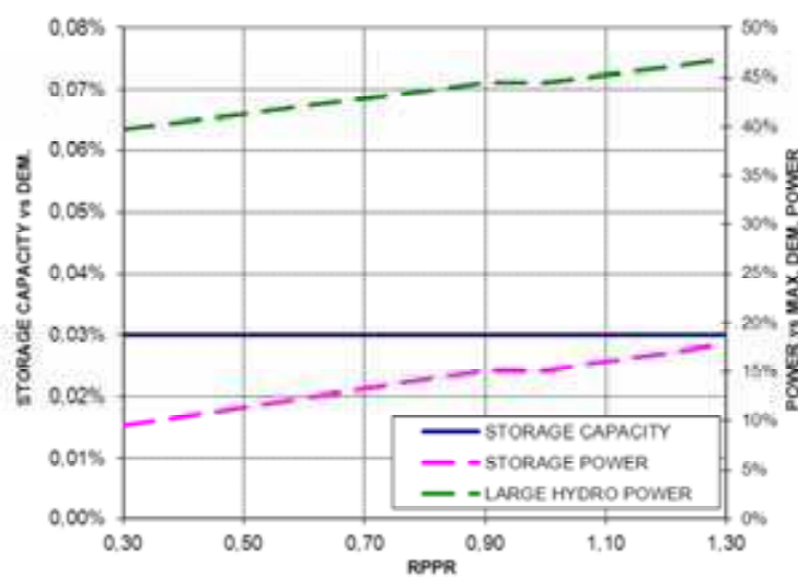
(b) Hydro empowered to 20 GW
