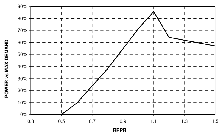
(b) Critical drives power curve
