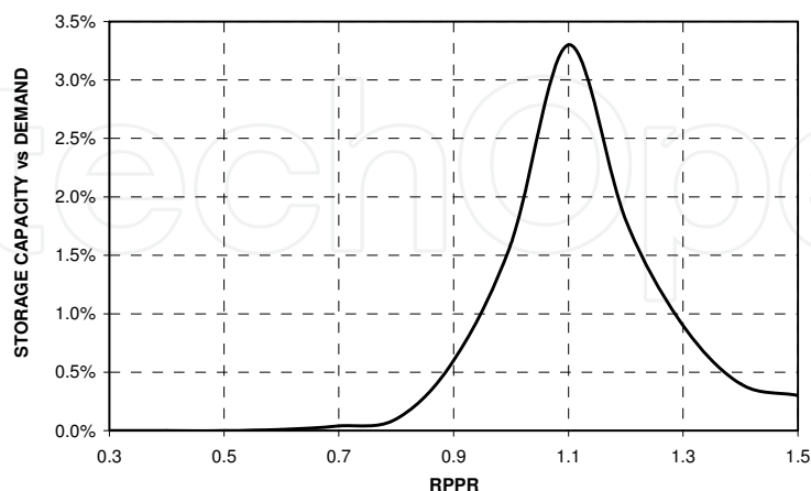
(a) Critical Storage Curve
