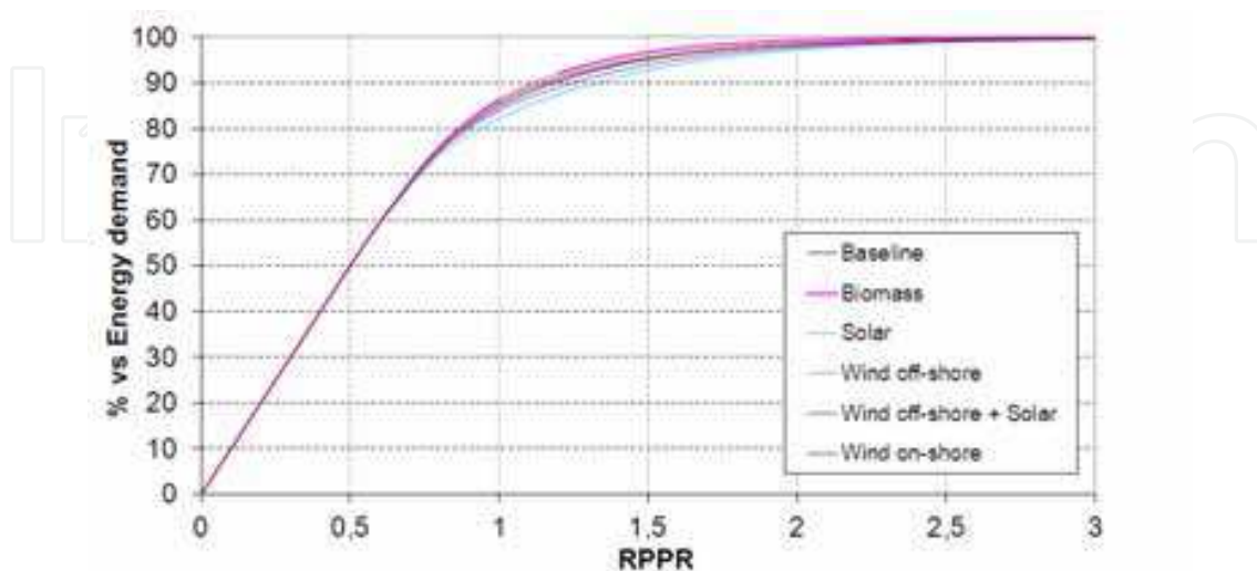
(a) Yearly Renewable production delivered to grid
