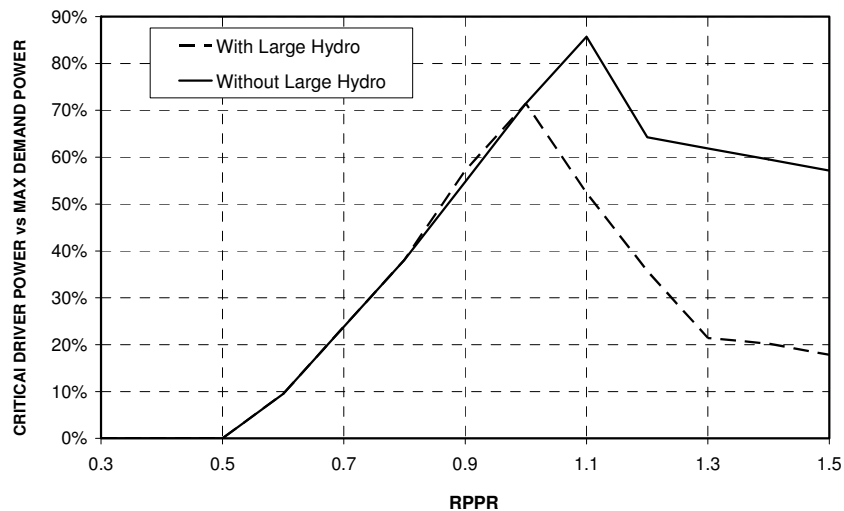
Fig. 15. Critical Power Drives for baseline case.
