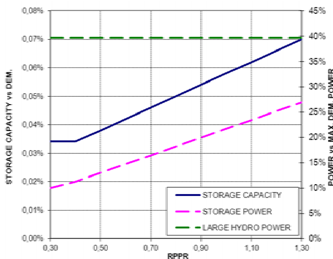
(a) No hydro empowering
