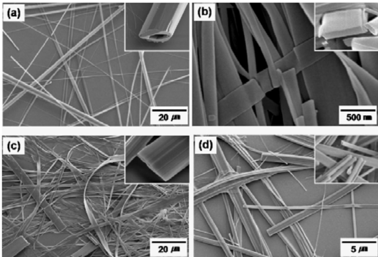
Fig. 4. Morphology of diverse nanostructures of the peptide formed in various solvents: (a) nanotubes formed in \text{H}_2\text{O} , (b) nanoribbons in \text{CH}_3\text{OH} , (c) nanoribbons in \text{C}_2\text{H}_5\text{OH} , and (d) nanoribbons and nanowires formed in \text{CH}_2\text{Cl}_2 (Han et al., 2008).
