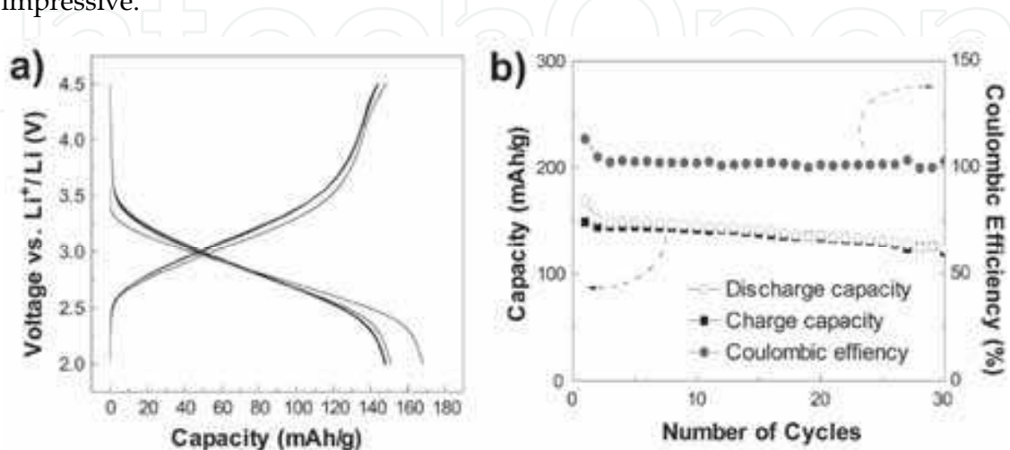
Fig. 25. (a) Discharge-charge profiles and (b) capacity retention of the amorphous \text{FePO}_4 nanotube at a current rate of 10 \text{ mA g}^{-1} (Ryu et al., 2010a).
