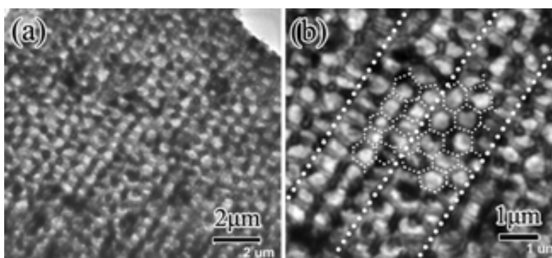
Fig. 28. TEM images of the butterfly wing-shaped \text{TiO}_2 photo-anode: (a) Medium resolution image and (b) high resolution image (Zhang et al., 2009).
