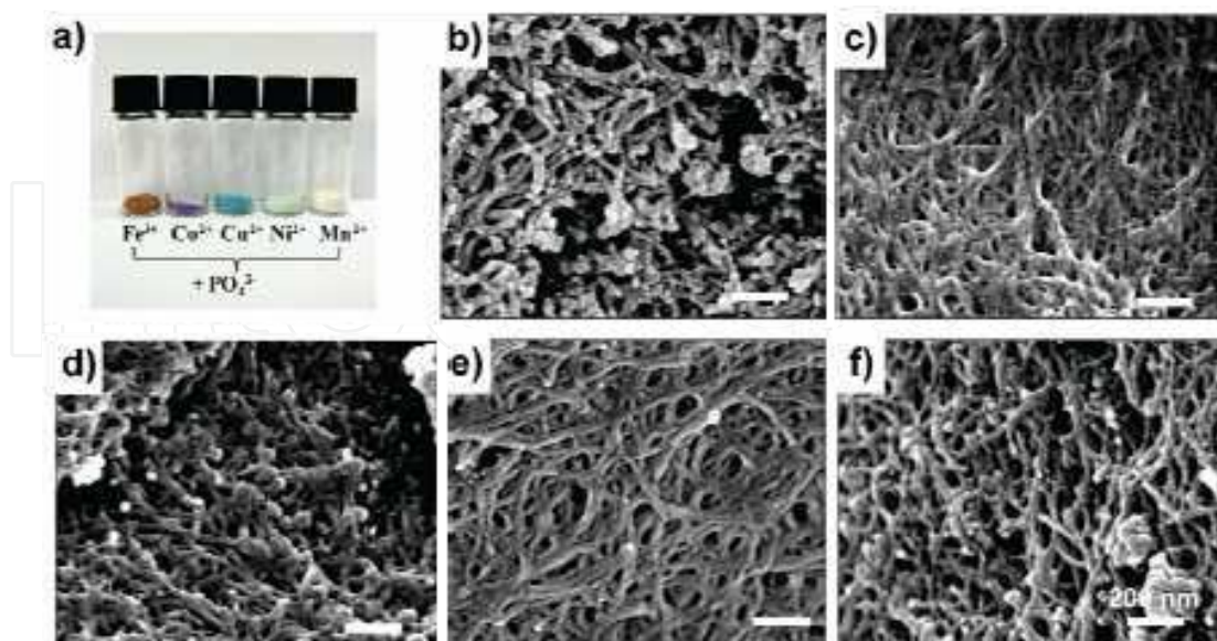
Fig. 23. (a) Photographs and (b-f) SEM images of various peptide-metal phosphate hybrid materials: injected metal ions are (b) \text{Fe}^{3+} , (c) \text{Co}^{2+} , (d) \text{Cu}^{2+} , (e) \text{Ni}^{2+} and (f) \text{Mn}^{2+} ions, respectively. (Ryu et al., 2010a).
