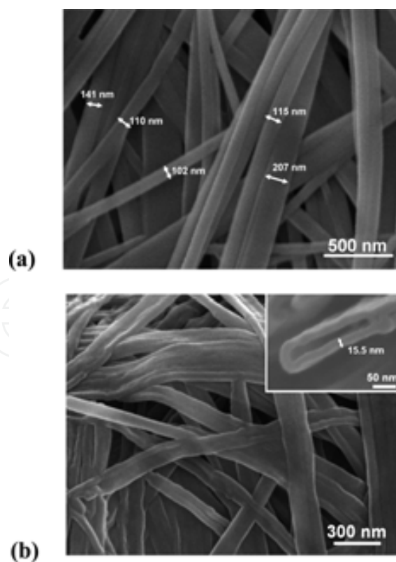
Fig. 20. SEM images of (a) the peptide template and (b) the \text{TiO}_2 nanotube network (inset: magnified cross-sectional image of \text{TiO}_2 nanotube) (Kim et al., 2009).
