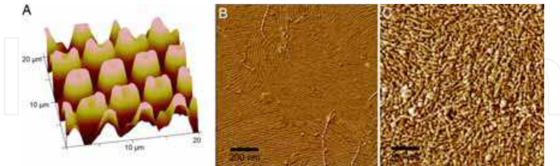
Fig. 12. AFM images of the virus-based microbattery: (a) height image of stacks of the virus- \text{Co}_3\text{O}_4 /(LPEI/PAA) multilayer/PDMS electrode, and phase image of the virus assembly onto the multilayer (b) before and (c) after the nucleation of \text{Co}_3\text{O}_4 (Nam et al., 2008).
