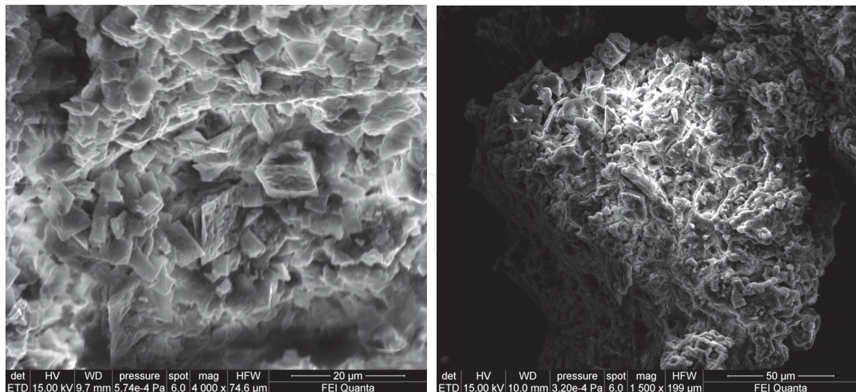
Fig. 5. SEM images of synthetic struvite
