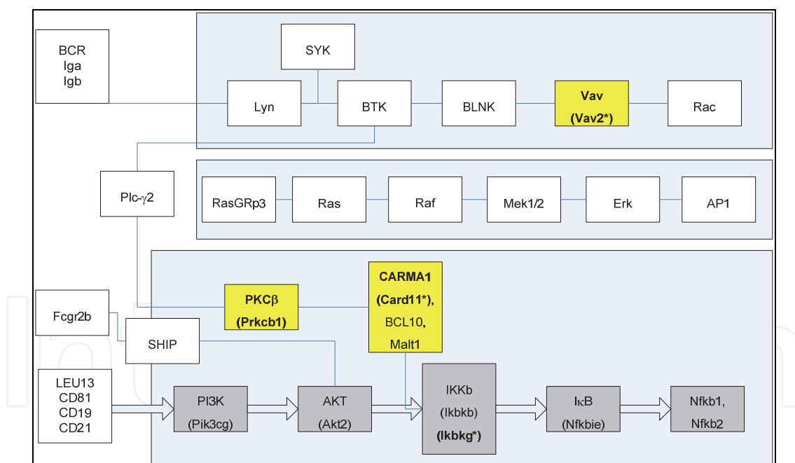
Fig. 5. Schematic representation of the BN+1 analysis results in the content of KEGG BCR pathway. The three blue boxes represent three major sub-networks within the BCR pathway with distinct regulatory and functional roles. The BN core network was defined using members from the third sub-network (dark grey boxes) which reflect major components of Nfkb signalling. Bolded gene names are those genes which were not included in the core network, yet were recovered during BN+1 analysis in the top 100 results. Note that not all members of the listed Nfkb signalling pathway were included in the core network (e.g. Ikbkg), and in some cases were not available on the microarray platform.
