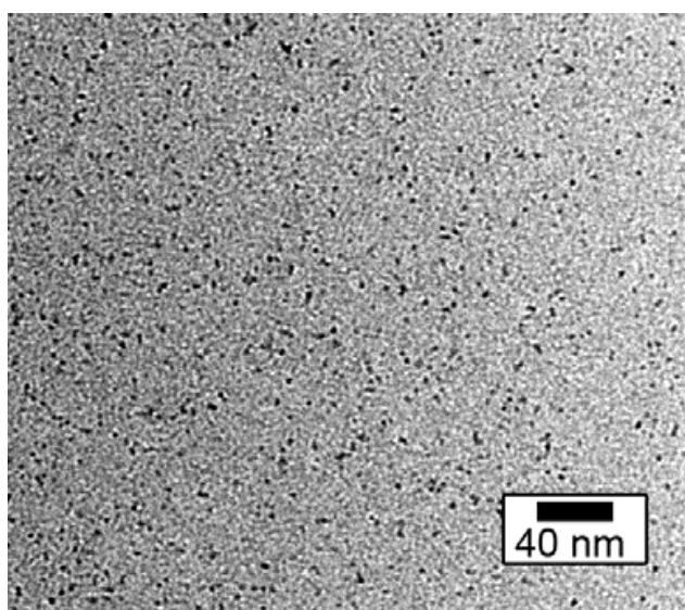
Fig. 7. TEM image of Ni nanoparticles immobilized in [\text{N}_{6,6,6}^+][\text{TA}^-] prepared via the indirect method, see text for details.
