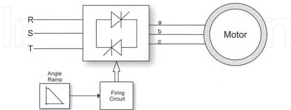
Fig. 3. Basic block diagram of the voltage-ramp technique.
