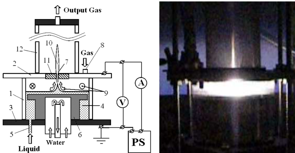
Fig. 27. Schematic (left) of the PLS reactor with the DC discharge in a reverse vortex gas flow of Tornado type with a "liquid" electrode and photo (right) of the TORNADO-LE working in ethanol-water solution.
