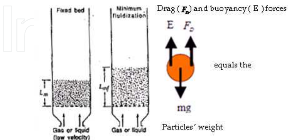
Fig. 8. Fixed and a fluidized bed of particles at a minimum fluidization velocity - adapted from (Kunii & Levenspiel, 1991).
