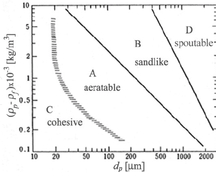
Fig. 4. Powder classification diagram for fluidization by air – source: (Geldart, 1972).
