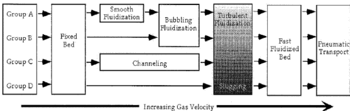
Fig. 5. Flow regime map for various powders.
