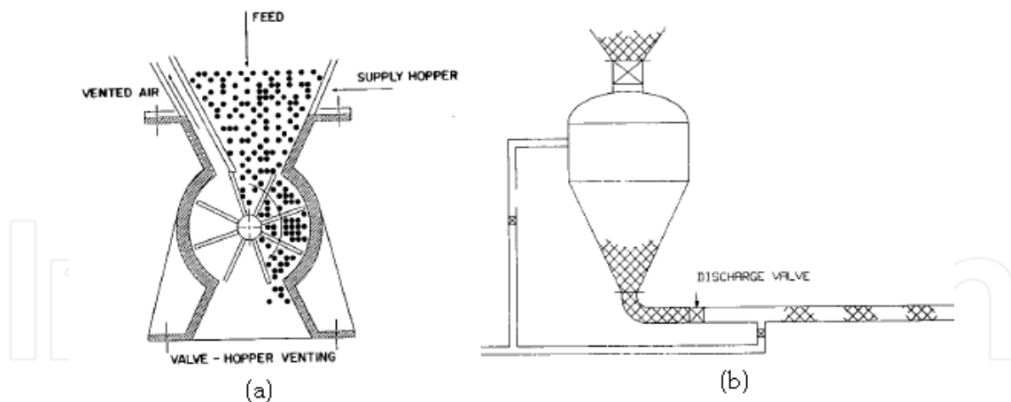
Fig. 12. Feeding devices used in pneumatic conveying of powders – source: (Klinzing et al , 1997).
