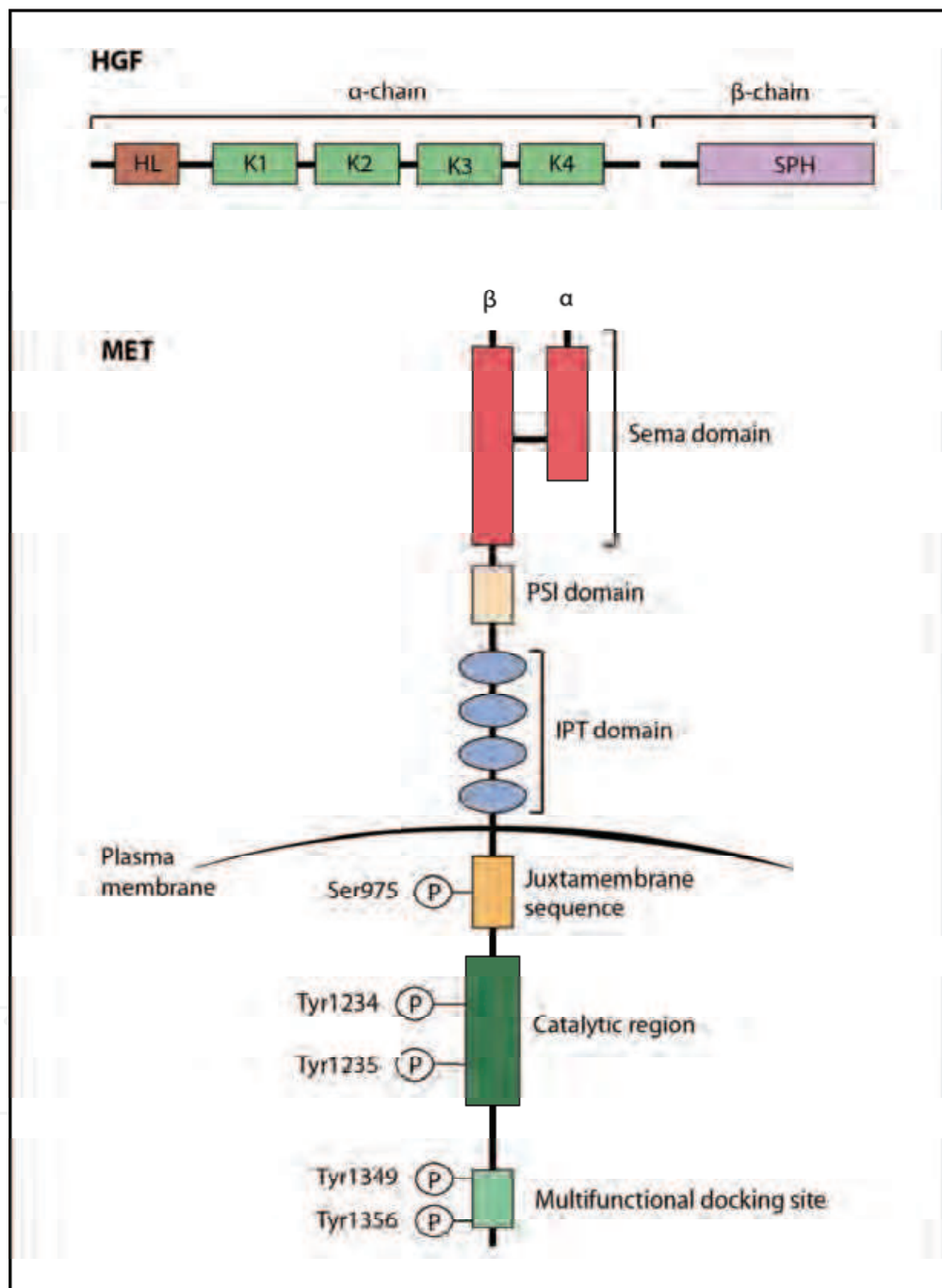
Fig. 1. HGF and Met structures
