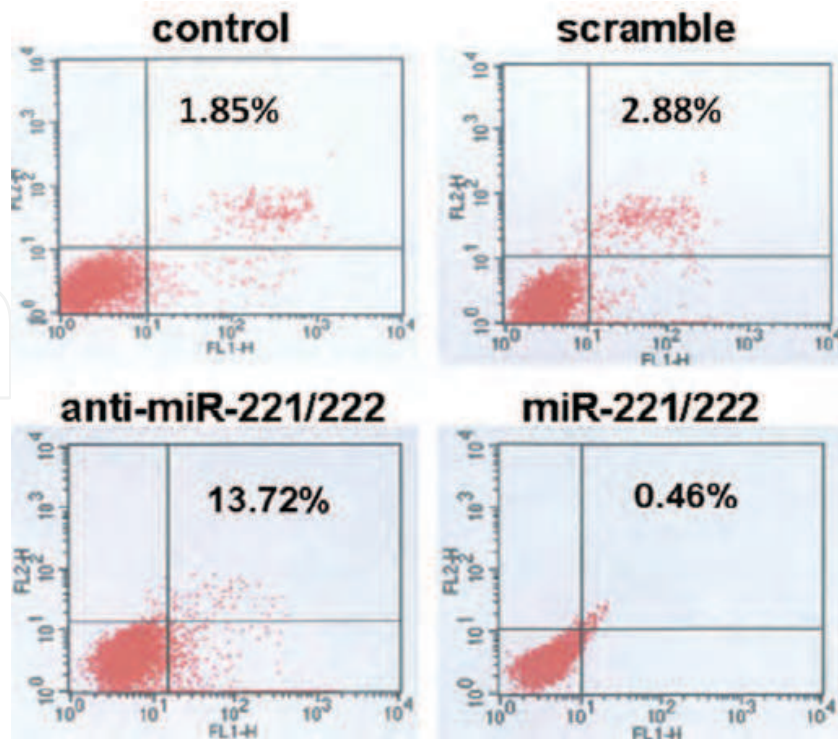
Fig. 4. Annexin V analysis showed that U251 cells transfected with As-miR-221/222 displayed significantly more apoptosis than the other three groups.
