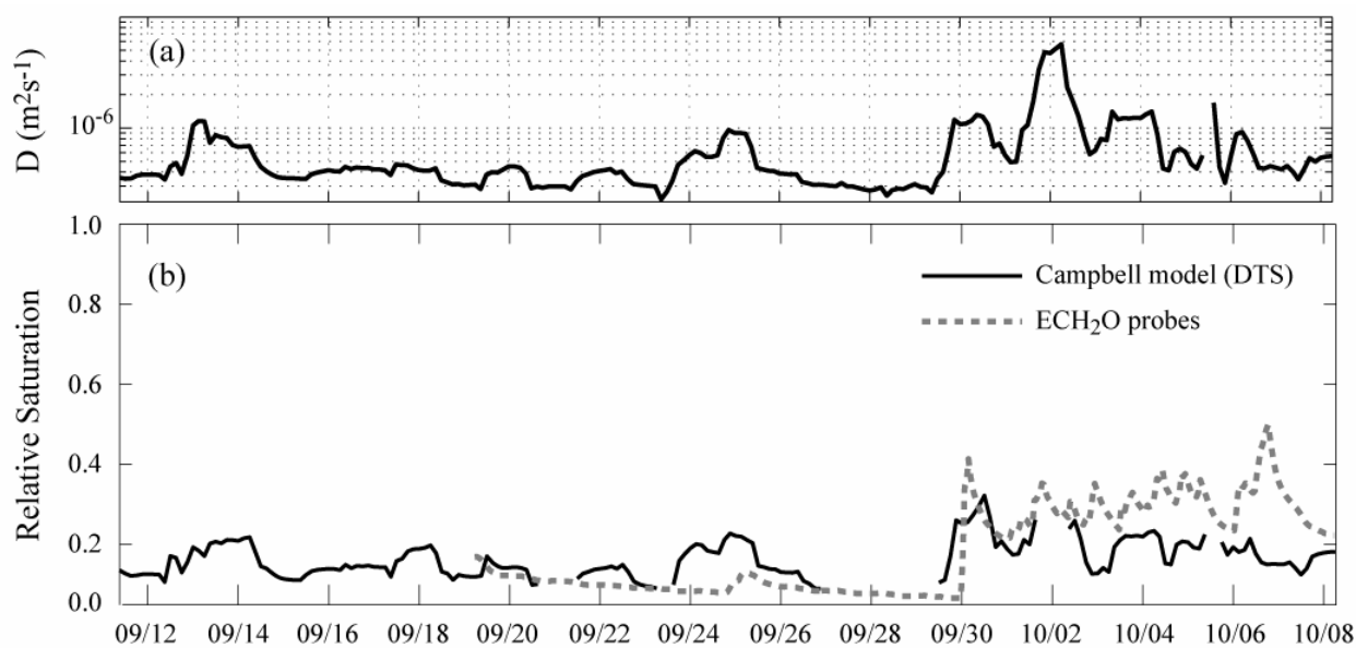
Fig. 10. (a) Estimated thermal diffusivity ( D ) at a selected location along the fiber-optic cable. (b) Mean value of relative saturation observed using ECH 2 O probes and inferred relative saturation from the estimated thermal diffusivity using the Campbell model (1985). Modified from Steele-Dunne et al. (2010)
