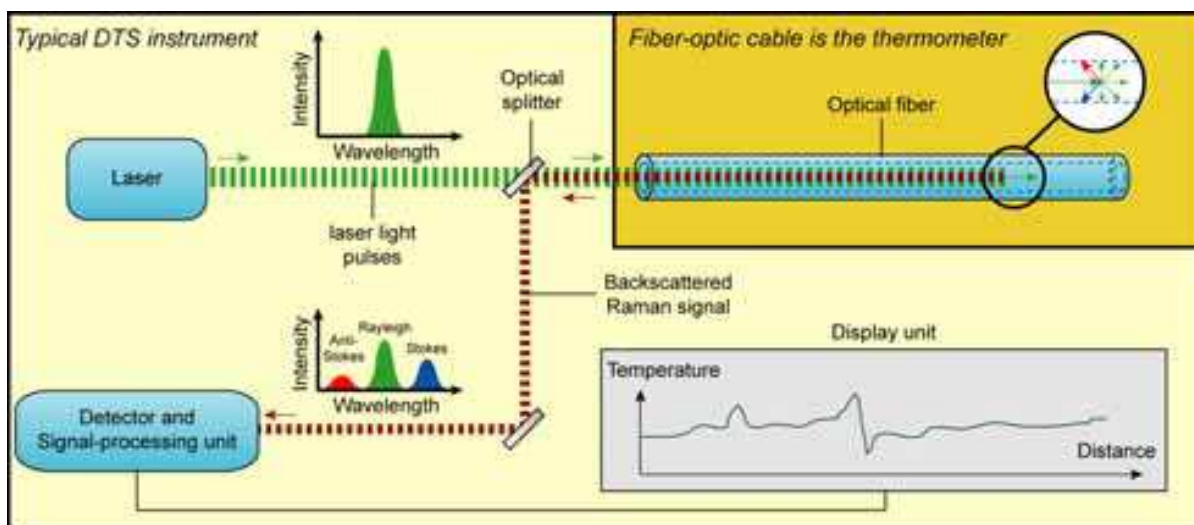
Fig. 4. Diagram of a typical distributed-temperature-sensing system
