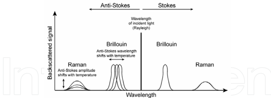
Fig. 3. Diagram of Rayleigh, Brillouin, and Raman backscattering in optical fibers
