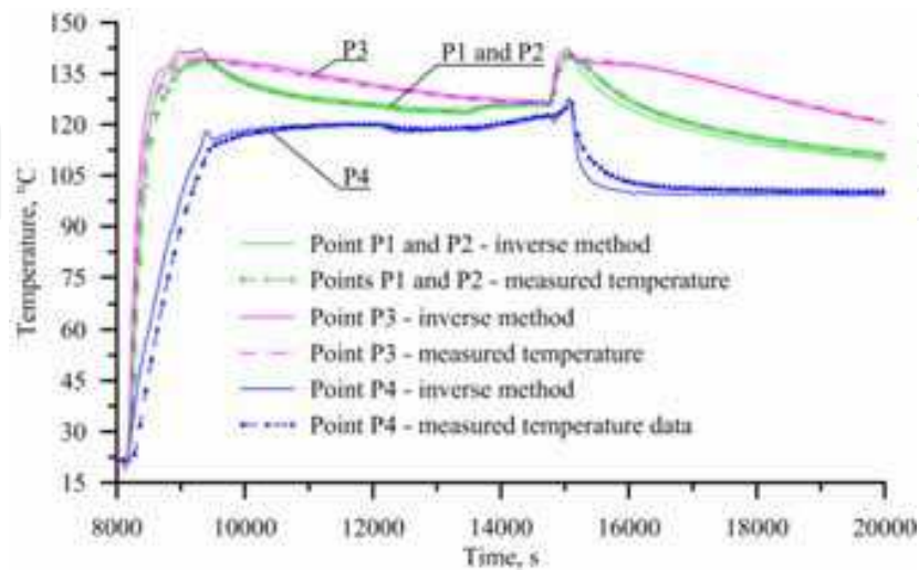
Fig. 15. Comparison of the calculated and measured time changes of the wall temperature at the interior points
