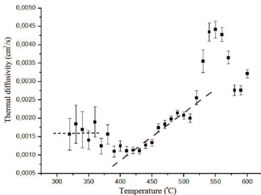
Fig. 6. Thermal diffusivity of dentin as function of temperature (Pereira et al., 2008)
