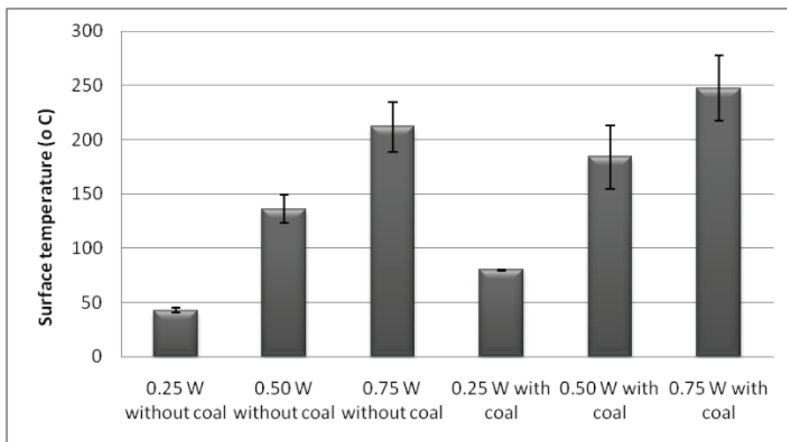
Fig. 8. Surface temperature increase on enamel surface during Er,Cr:YSGG ( \lambda = 2078 nm) laser irradiation with and without the application of coal paste (Ana et al., 2007). It can be noted that, even at three different average powers, the presence of the photosensitizer significantly increased the surface temperature during laser irradiation. Bars mean standard deviation
