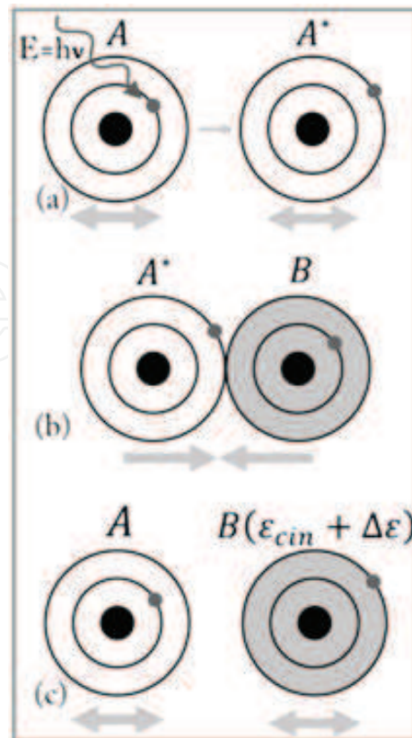
Fig. 2. Schematic diagram of the heat generation in a biological tissue: (a) a photon with the energy h\nu is applied in the molecule A , then goes to an excited state A^* . (b) The molecule A^* collides with B . (c) A^* transfers its energy to B ; B becomes B(\epsilon_{cin} + \Delta\epsilon) and starts to vibrate more intensely
