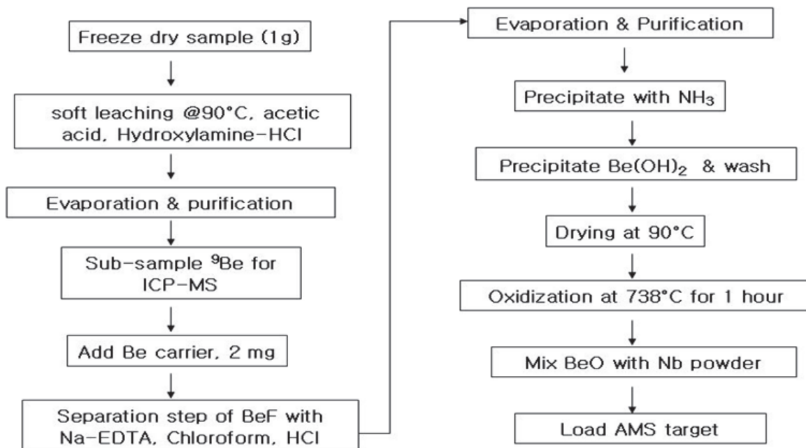
Fig. 3. Description of authigenic Be isotope extraction method.
