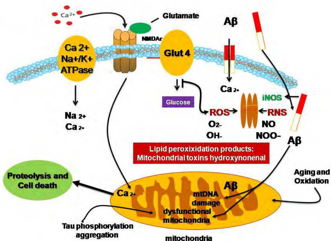
Fig. 1. Oxidative distress
