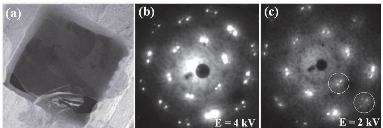
Fig. 17. The SEM image of folding double graphene sheet (a) and its LETED pattern at (b) 4 kV and (c) 2kV.
