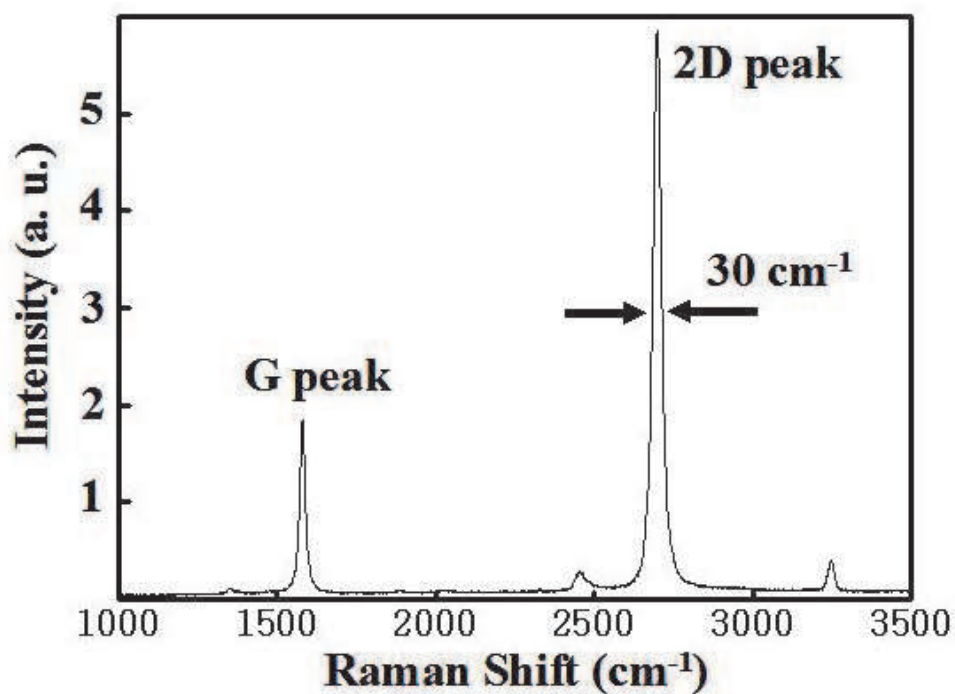
Fig. 14. Typical Raman spectrum of the monolayer self-standing graphene sheets. Small defect-origin D peak was detected at \sim 1350 \text{ cm}^{-1} .
