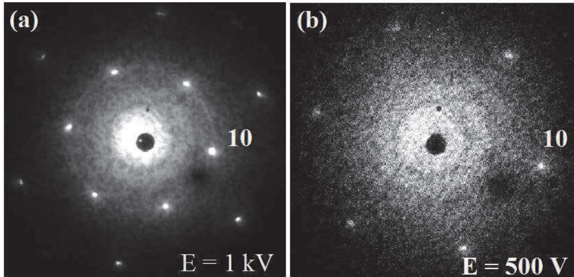
Fig. 16. The LETED pattern of single-layer graphene at (a) 1 kV and (b) 500 V.
