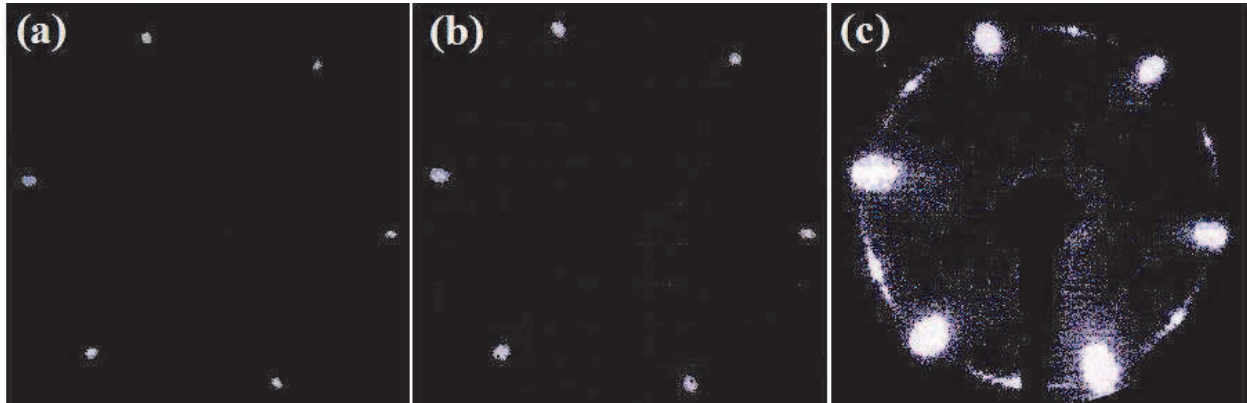
Fig. 8. Typical LEED patterns of (a) h-BN/Ni(111) and (b), (c) graphene/h-BN/Ni(111). The pattern (c) was obtained for a longer exposure, while the pattern of (b) was measured for normal exposure.
