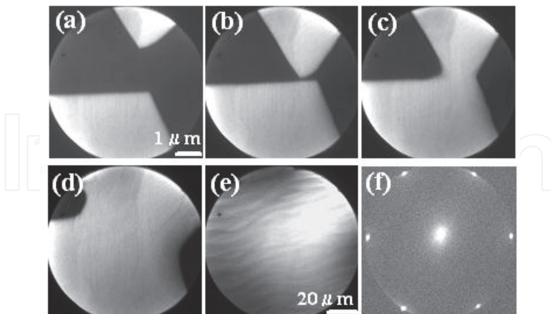
Fig. 6. Typical snapshots of LEEM images obtained as the temperature was decreased from 1200 K to 1125 K (images (a) to (d)). The observed area was 6\mu\text{m} field-of-view. Letter in each image indicates the time-lapse order. Two graphene domains were united to form one graphene sheet. Image (e) is a typical LEEM image of 100\mu\text{m} field-of-view. The surface was entirely covered with monolayer graphene. LEEM images were obtained at the primary electron energy of 3.5 eV. Image (f) is a typical \mu\text{LEED} pattern observed in the graphene-covered surface. The orientation of the graphene was slightly altered because the sheet is curved.
