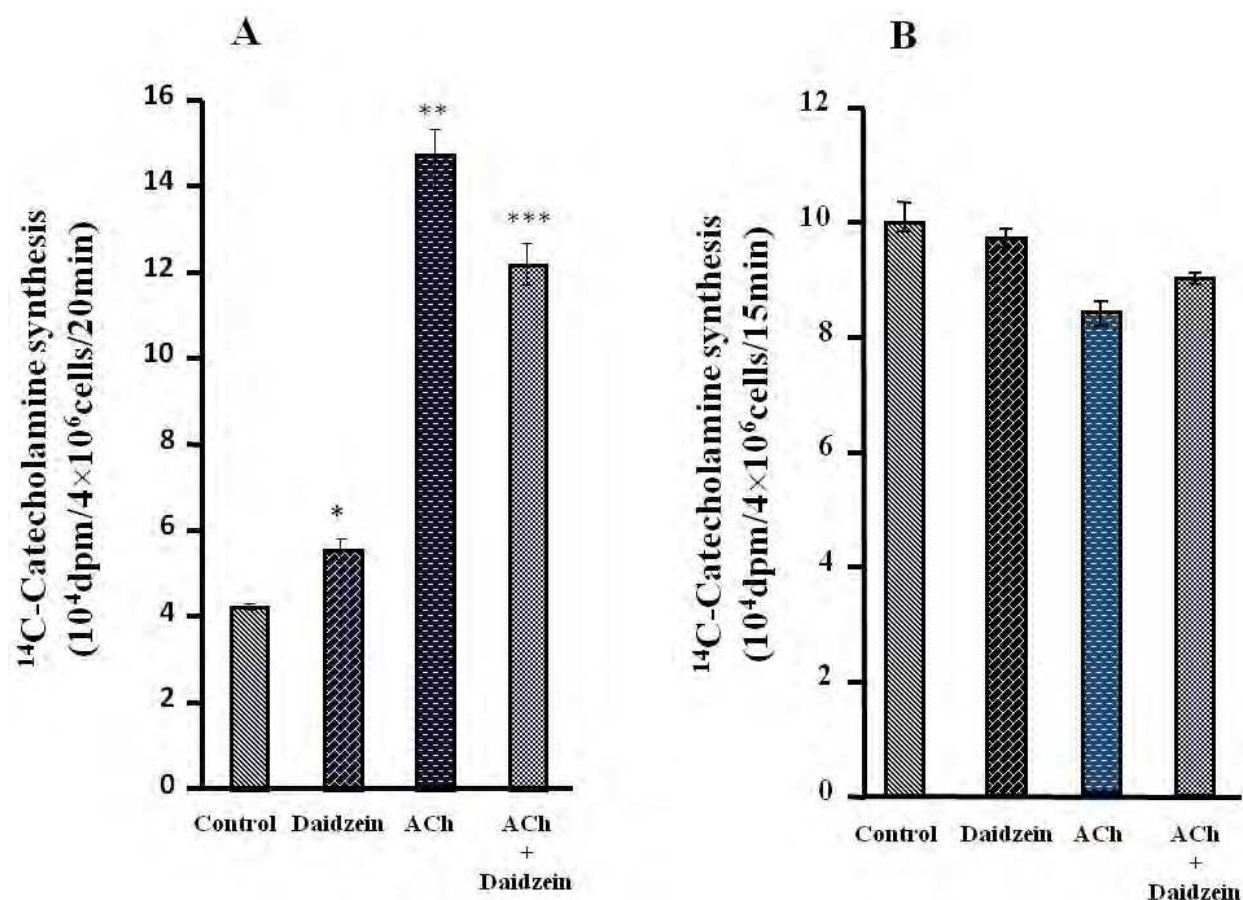
Fig. 2. Effects of daidzein on 14 C-catecholamine synthesis from [ 14 C]tyrosine (A) or [ 14 C]DOPA (B). The cells (4 × 10 6 /dish) were incubated with or without daidzein (1 μM) and acetylcholine (ACh)(0.3 mM) at 37 °C for 20 min or 15 min in the presence of L-[U- 14 C]tyrosine (20 μM, 1 μCi) (A) or [ 14 C]DOPA (20 μM, 0.25 μCi) (B), respectively. The 14 C-catecholamines formed were measured. Data are expressed as the mean ± SEM of four experiments carried out in triplicate. * p < 0.05 and ** p < 0.01, compared with control; *** p < 0.05, compared with acetylcholine alone. Data from Liu et al. (2007) are modified.
