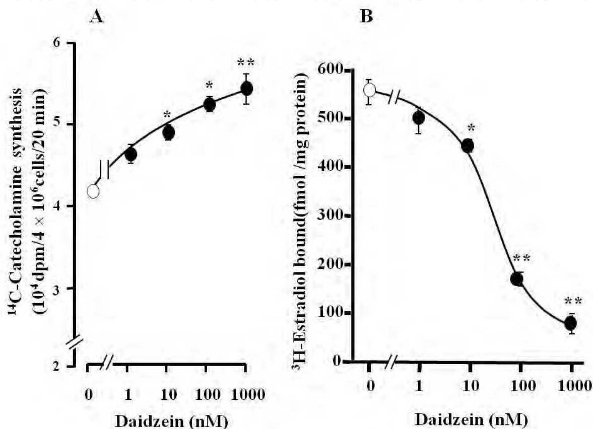
Fig. 1. Concentration–response curve of daidzein for ^{14}\text{C} -catecholamine synthesis from ^{14}\text{C} tyrosine in cultured bovine adrenal medullary cells (A) and concentration-inhibition curve for specific binding of ^3\text{H} 17 \beta -estradiol to adrenal medullary plasma membranes (B). (A) Cultured bovine adrenal medullary cells ( 4 \times 10^6 / dish) were incubated with (●) or without (○) various concentrations (1 – 1000 nM) of daidzein at 37 °C for 20 min in 1.0 ml KRP buffer containing L-[U- ^{14}\text{C} ]tyrosine (20 \mu\text{M} , 1 \mu\text{Ci} ). The ^{14}\text{C} -labeled catecholamines formed are measured and shown as the total ^{14}\text{C} -catecholamines (adrenaline, noradrenaline and dopamine). Data are expressed as the mean \pm SEM of four experiments carried out in duplicate. * p < 0.05 and ** p < 0.01 , compared with control. (B) Plasma membranes isolated from bovine adrenal medulla were incubated at 4 °C for 30 min with various concentrations of daidzein in the presence of ^3\text{H} 17 \beta -estradiol (5 nM, 0.1 \mu\text{Ci} ). Non-specific binding was determined in the presence 1 \mu\text{M} of 17 \beta -estradiol and specific binding was obtained by subtracting non-specific binding from total binding. Values shown are means \pm SEM of four separate experiments carried out in triplicate. * p < 0.05 and ** p < 0.01 , compared with control. Data from Liu et al. (2007) are modified.
