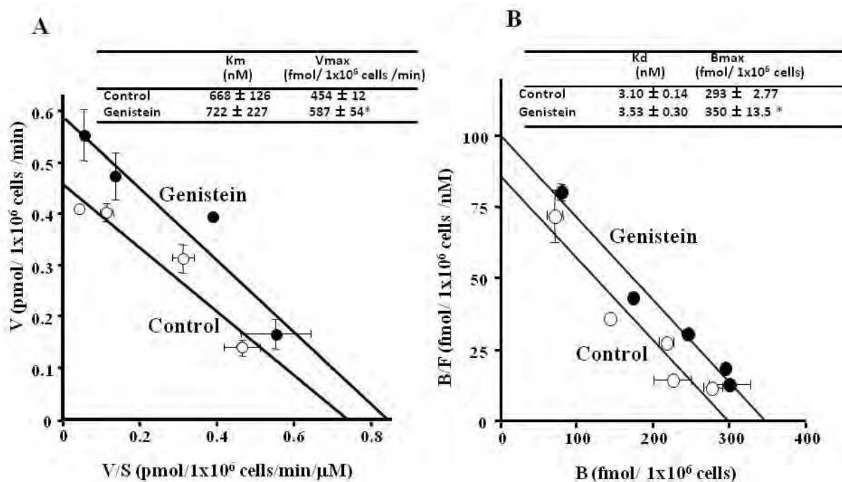
Fig. 6. Eadie-Hofstee plots of [ ^3 H] noradrenaline uptake (A) and Scatchard plots of specific [ ^3 H]nisoxetine binding (B) in bovine noradrenaline transporter transfected COS-7 cells. (A) Cells were pretreated with or without genistein (10 \mu M) for 20 min at 37 ^{\circ} C. Desipramine-sensitive [ ^3 H] noradrenaline uptake was measured with various concentrations (0.1 - 10 \mu M) of [ ^3 H] noradrenaline and analyzed by Eadie-Hofstee method of [ ^3 H] noradrenaline uptake. Data are means \pm SEM from three separate experiments. Inset: V_{max} and K_m values were calculated by Eadie-Hofstee analysis of the saturation curves in the absence (control) or presence of 10 \mu M genistein. * p < 0.05, compared with control. (B) The bovine noradrenaline transporter transfected COS-7 cells were incubated with increasing concentrations of [ ^3 H]nisoxetine (1 - 24 nM) in the presence or absence of genistein (10 \mu M) at 4 ^{\circ} C for 2 h. Non-specific binding was determined in the presence of 10 \mu M nisoxetine. The specific binding was 30-40% of the total binding at the K_d concentration of [ ^3 H]nisoxetine. The data are plotted by Scatchard plot analysis of the saturation curves of [ ^3 H]nisoxetine specific binding in the absence (control) or presence of 10 \mu M genistein. Data are means \pm SEM from three separate experiments. * p < 0.05, compared with control. Data from Toyohira et al. (2010) are modified.
