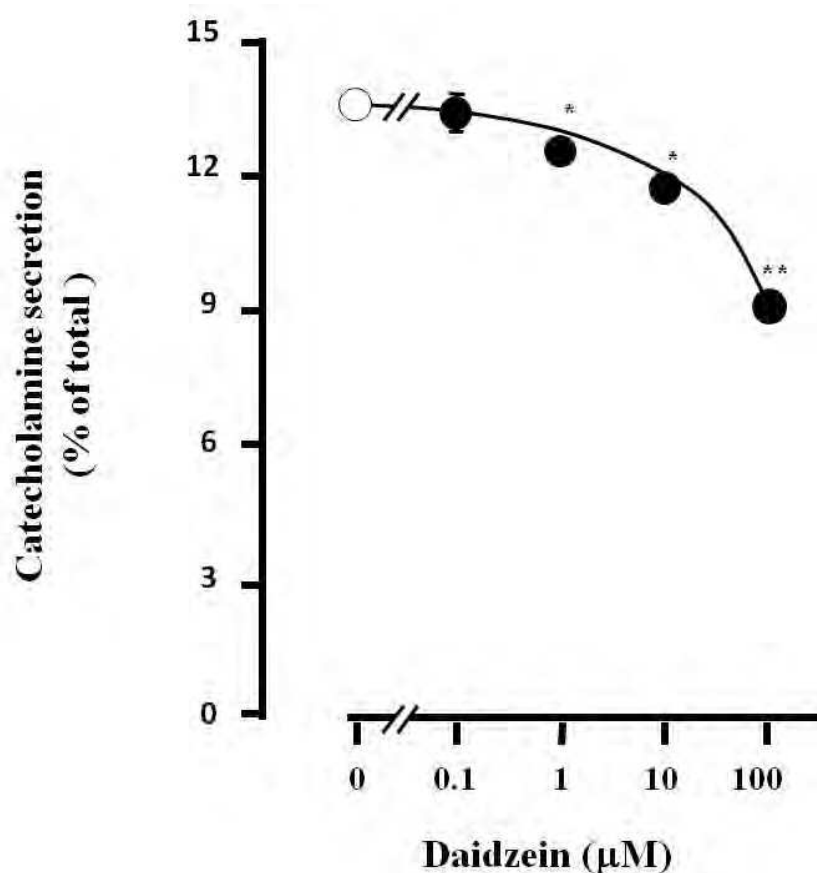
Fig. 4. Effects of daidzein on catecholamine secretion induced by acetylcholine in bovine adrenal medullary cells. Cells ( 2 \times 10^6 /dish) were incubated with acetylcholine (0.3 mM) in the presence (●) or absence (○) of various concentrations (0.1-100 \mu M) of daidzein for 10 min at 37 °C. Catecholamines secreted into the medium were measured, and expressed as percentage of total catecholamines. Data are means \pm SEM of four experiments carried out in duplicate. * p < 0.05 , compared with control (0 \mu M daidzein). Data from Liu et al. (2007) are modified.
