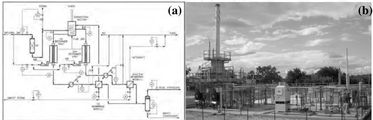
Fig. 6. Process scheme (a) and bird-eye view (b) of the industrial test plant
