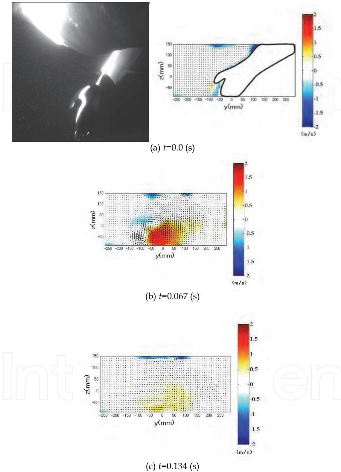
Fig. 17. Flow field in the y - z plane obtained through the stereoscopic PIV method. The vectors denote the velocities in the plane, while the colors represent the magnitude induced by the hand motion opposite to the swimming direction, i.e., the x -direction.
