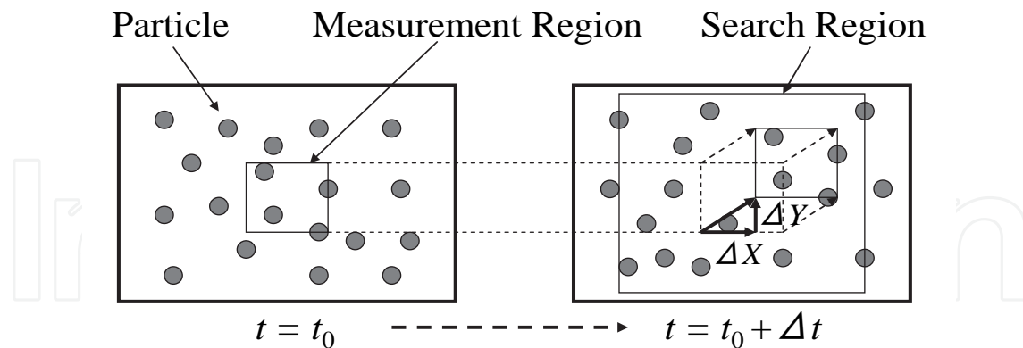
Fig. 3. Principle of determining velocity through PIV.
