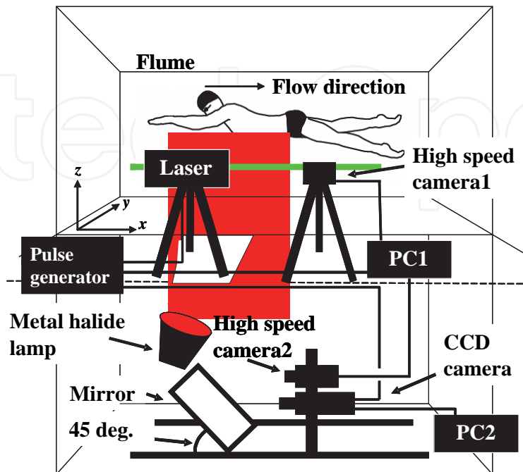
Fig. 4. Experimental configuration and setup.
