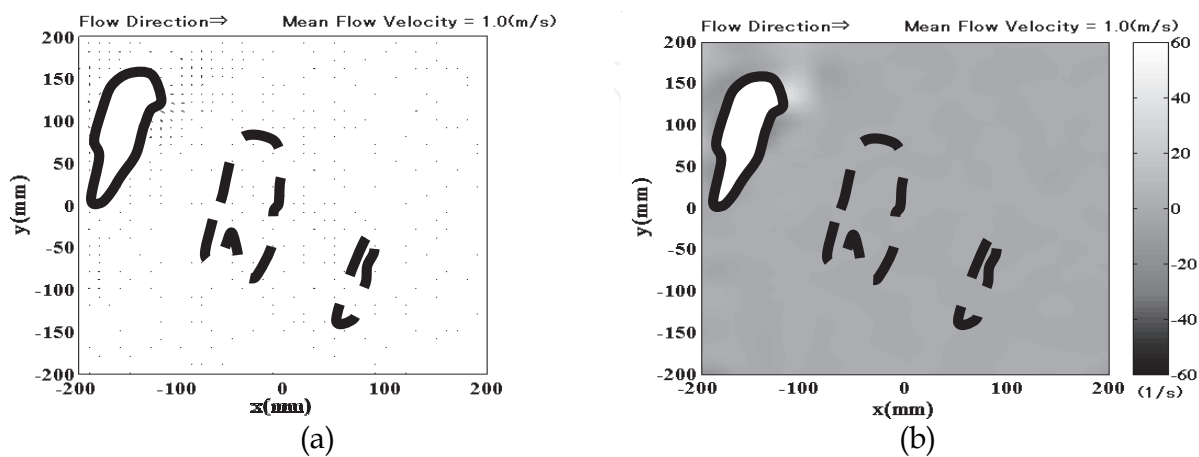
Fig. 14. Velocity (a) and vorticity (b) fields at 0.036 s are shown. The solid line corresponds to the outline of the hand at this instant and the other two broken lines show the outlines at instants 0.068 s and 0.136 s later.
