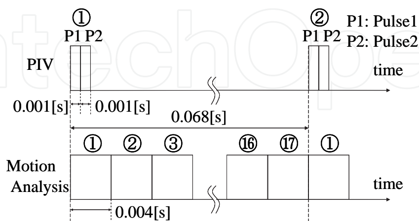
Fig. 7. Timing chart of the dual analysis system. The time interval used for obtaining the flow field using PIV was set at 68 ms, while the motion analysis using high-speed cameras set at 4 ms.
