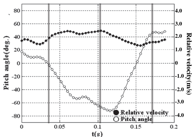
Fig. 11. Variations of pitch angle and hand velocity. The three vertical lines drawn in bold indicate instants of 0.036, 0.104, and 0.172 s
