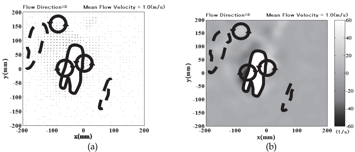
Fig. 15. Velocity (a) and vorticity (b) fields in the x - y plane at 0.104 s. The solid line corresponds to the outline of the hand cross section at this instant and the two broken lines show the outlines at 0.036 s and 0.172 s. The three circles with arrows indicate the vortices.
