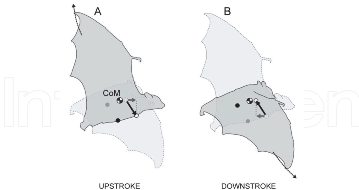
Fig. 1. Effect of the oscillation of the wings on the position of the center of mass (COM) and accelerations of the body. When external forces, such as aerodynamic and gravitational forces, are absent, the position of the COM will remain constant but the body moves in opposition to the flapping wings to conserve momentum. Closed and open symbols correspond to the pelvis and chest markers, respectively. During upstroke (A), the upward and backward acceleration of the wings will produce an inertial force (black arrow) that will move the body forward and downward with respect to the downstroke. This force will produce a forward-oriented component, or inertial thrust, during upstroke (grey arrow). During downstroke (B), the downward and forward acceleration of the wings will produce an inertial force (black arrow) that will move the body backward and upward while keeping the position of the COM constant. The horizontal component of this inertial force will produce negative inertial thrust during downstroke (grey arrow).
